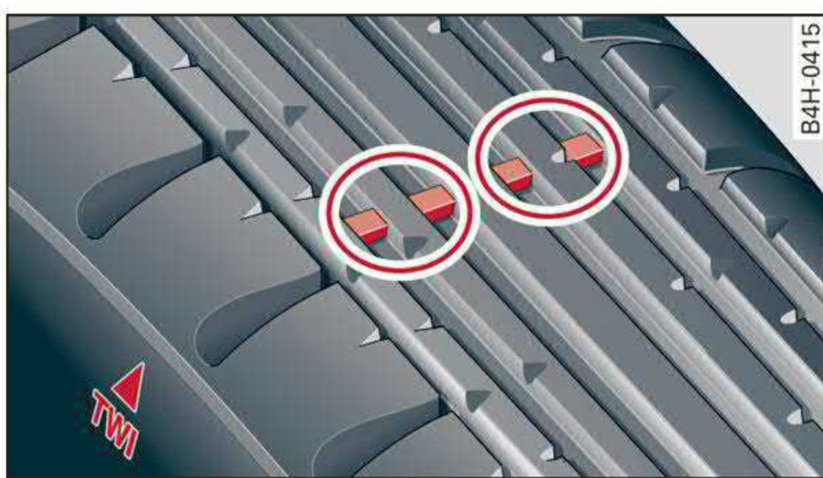
Fig. 153 Tire profile: treadwear indicator
