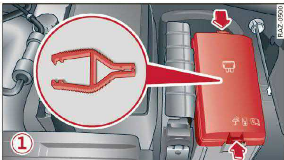
Fig. 169 Left side of the engine compartment: fuse cover ①
