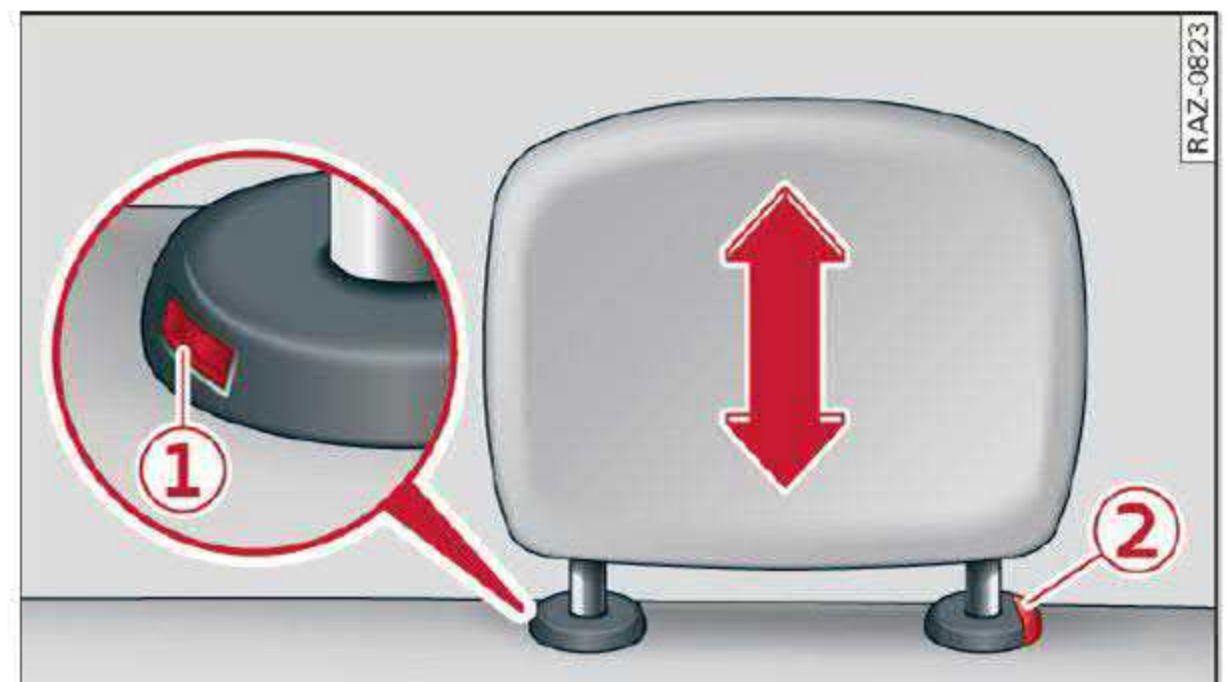
Fig. 56 Rear seat: operating the head restraints
