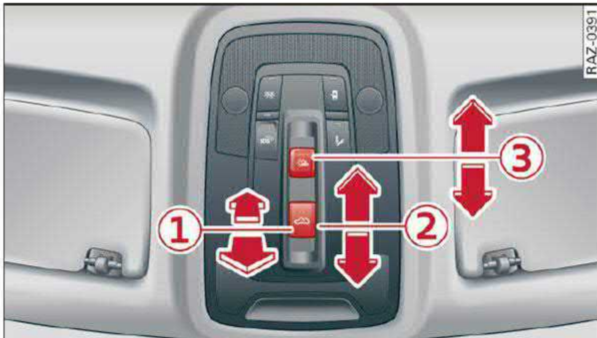
Fig. 35 Headliner: panoramic glass roof and sunshade* buttons
