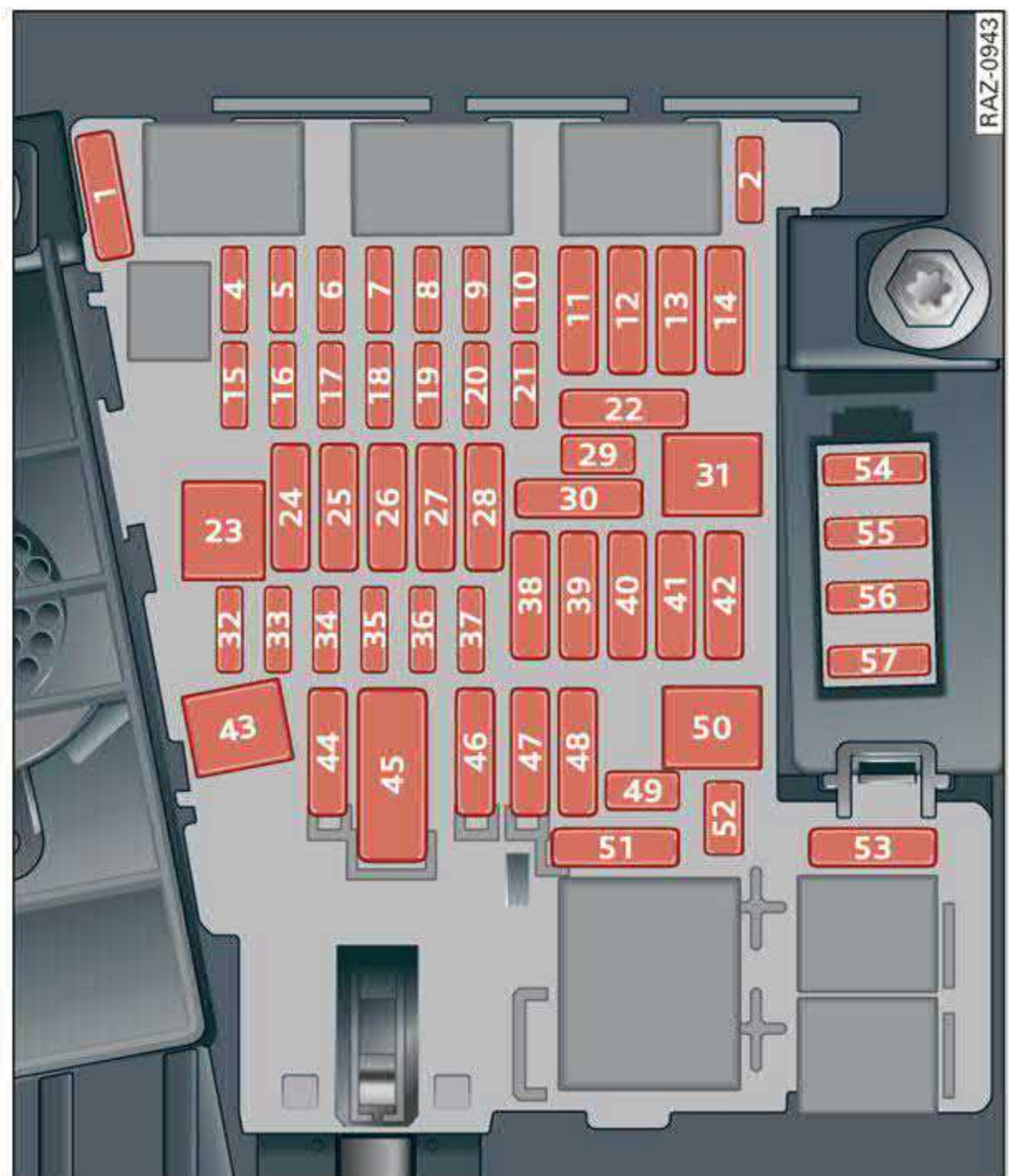
Fig. 172 Left side of cockpit: fuse assignment
