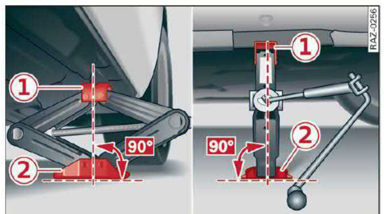
Fig. 161 Sill: positioning the vehicle jack
