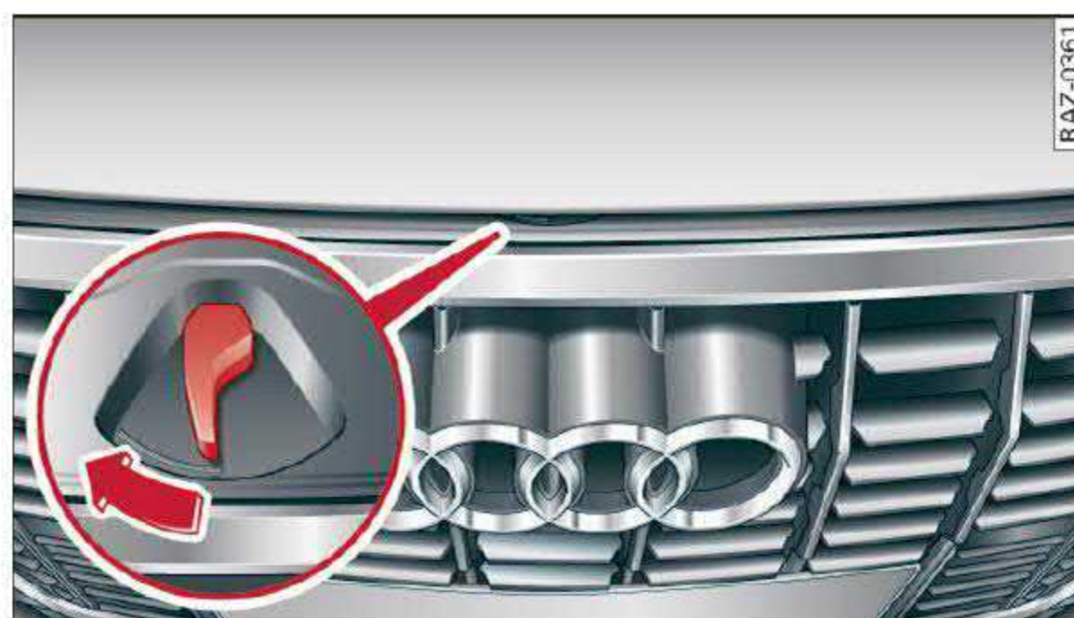
Fig. 144 Unlocked hood: lever
