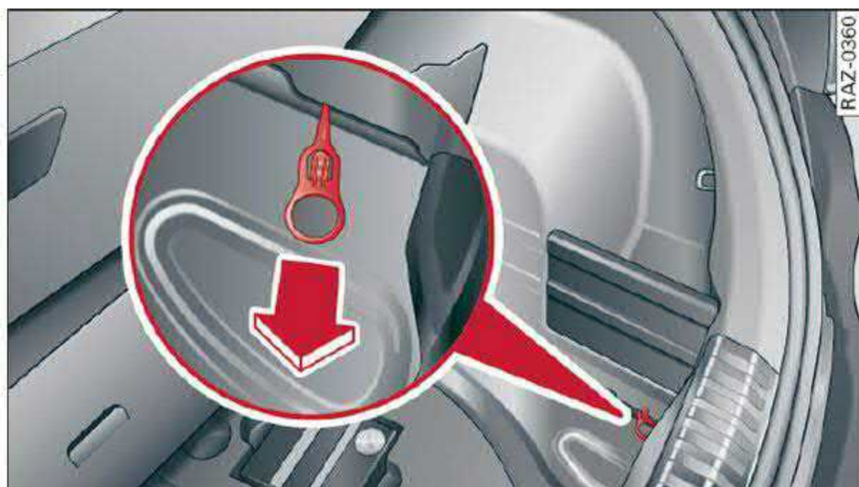
Fig. 142 Luggage compartment: fuel filler door emergency release
