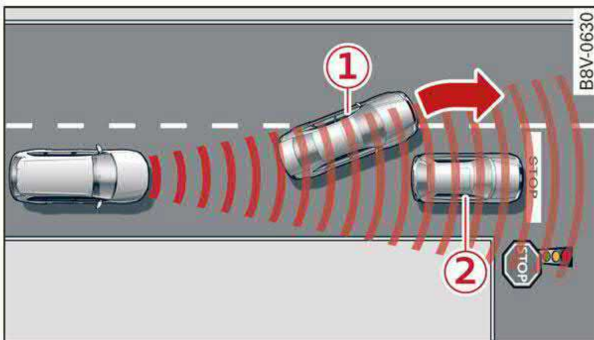
Fig. 92 Example: vehicle changing lanes and stationary vehicle
