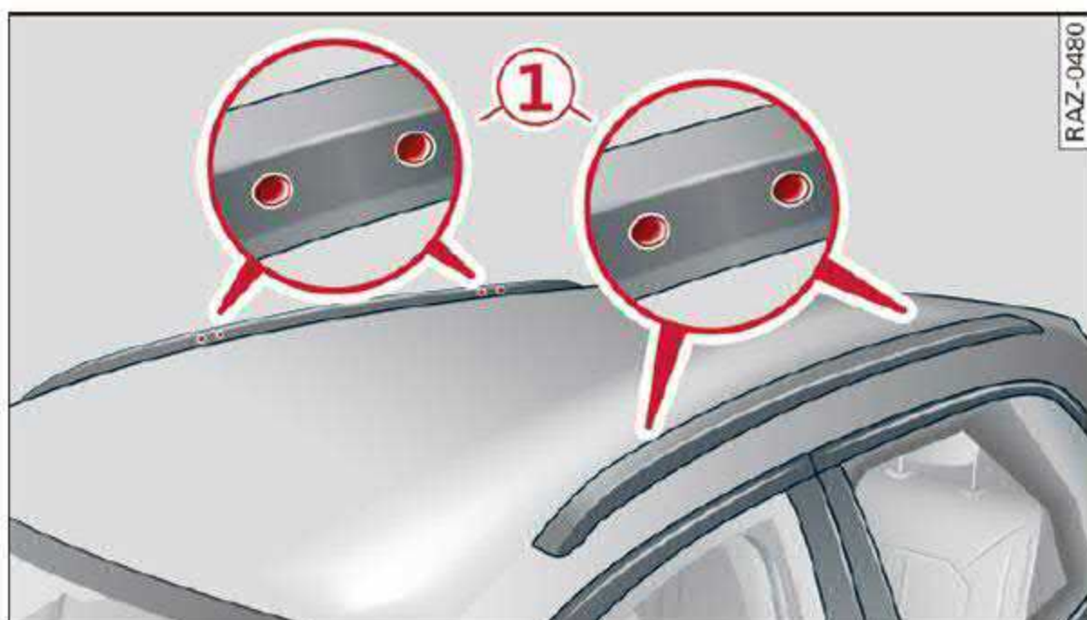
Applies to: vehicles with roof rail Fig. 76 Roof rail: mounting points
