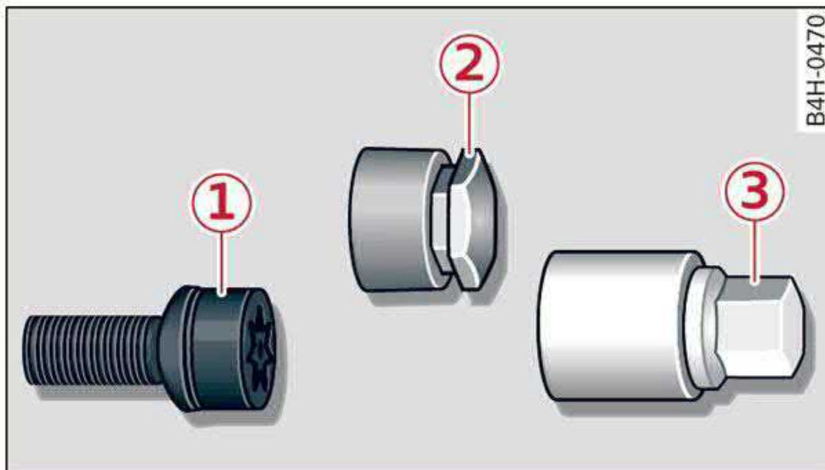
Fig. 158 Anti-theft wheel bolt with cap and adapter
