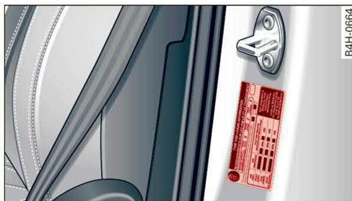
Fig. 154 Driver's side B-pillar: tire pressure label
