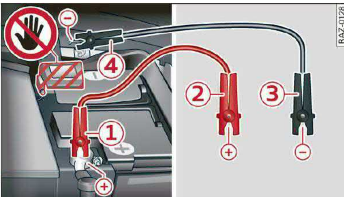
Fig. 166 Connecting the jump start cables
