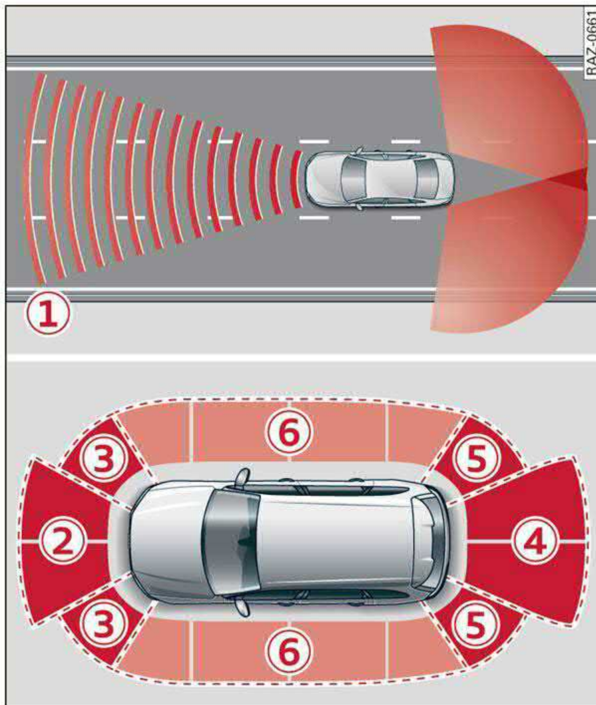
Fig. 85 Sensor coverage area
