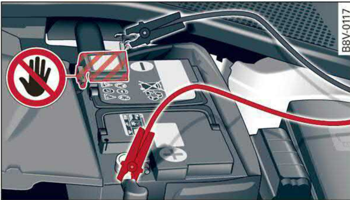
Fig. 165 Engine compartment: connectors for jump start cables or a charger
