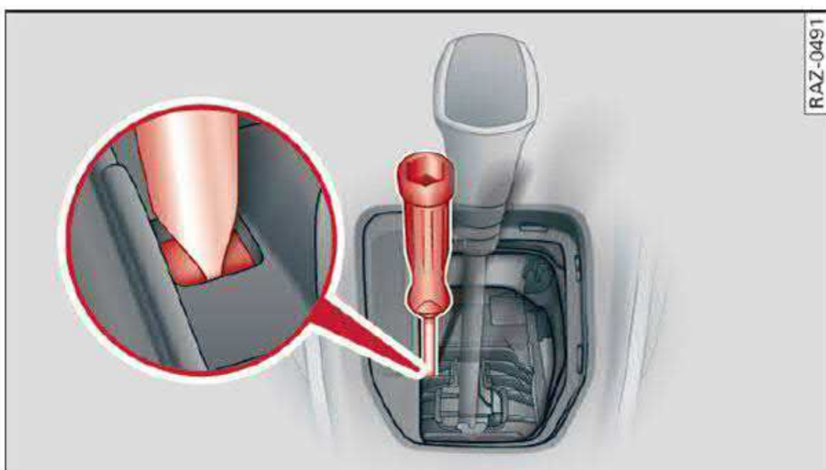
Fig. 84 Selector lever: releasing the parking lock using the emergency release
