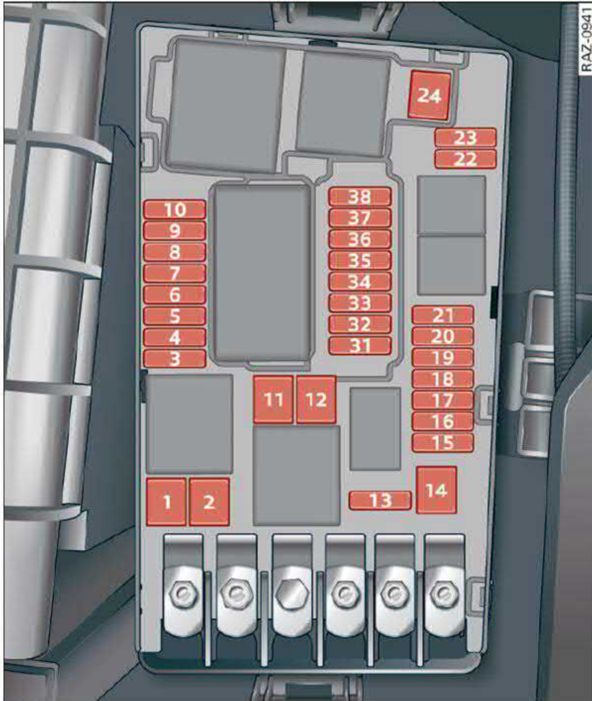
Fig. 171 Left side of engine compartment: fuse assignment
