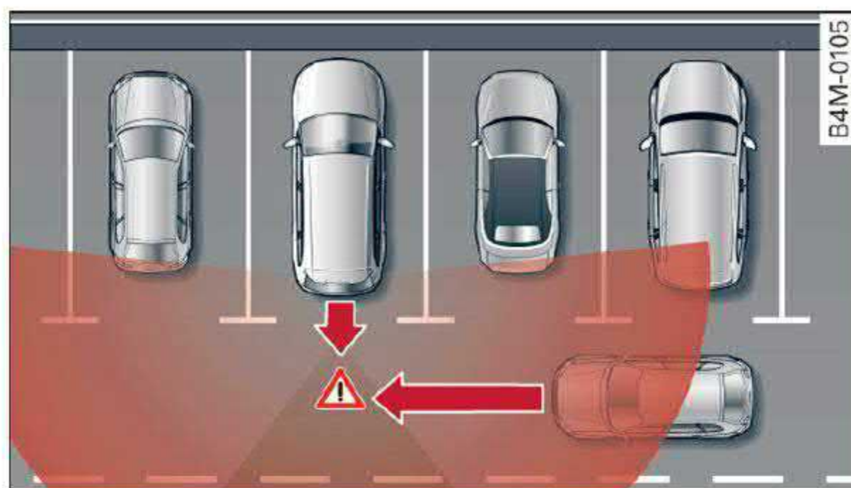
Fig. 115 Sensor detection range for rear cross-traffic assist
