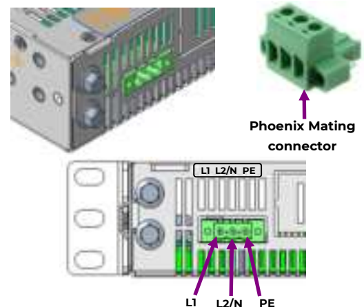
Figure 8: AC Input Terminal block Connector
