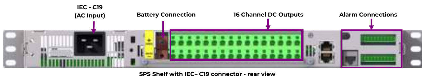
Figure 1: SPS Shelf front and rear view
