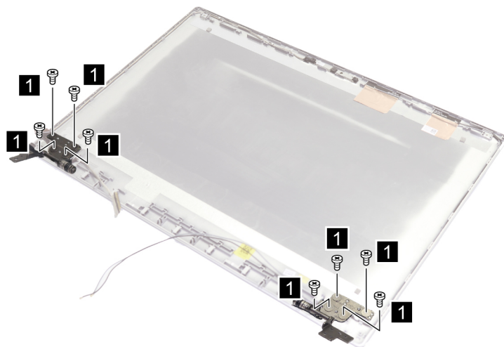
Figure 47. Remove 8 screws
