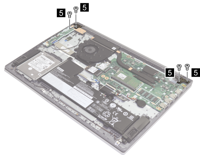
Figure 36. Remove four screws
