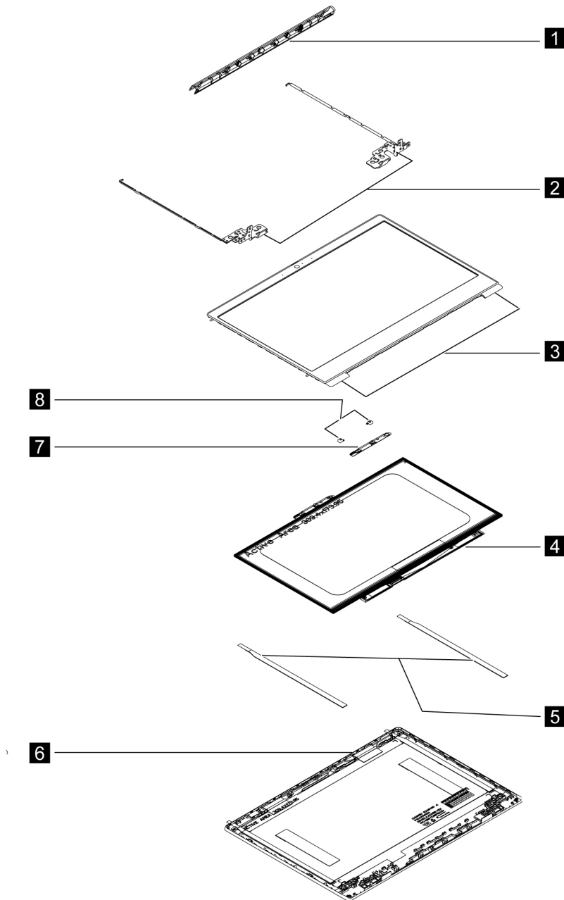
Figure 1. 14-inch and 15-inch models LCD exploded view
