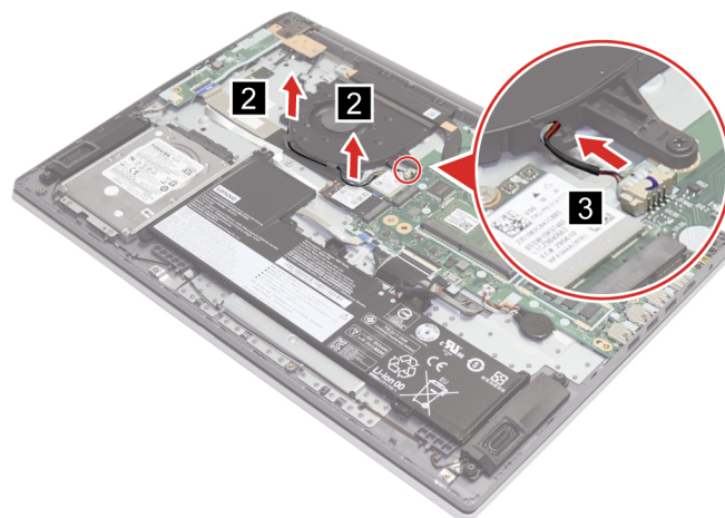
Figure 16. Disconnect the fan cables
