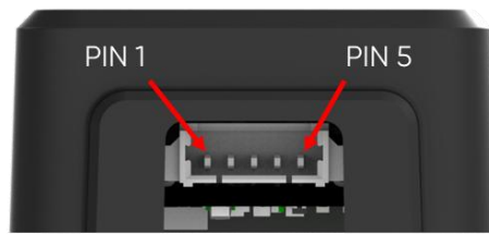
Figure. 5: LiDAR connector appearance
