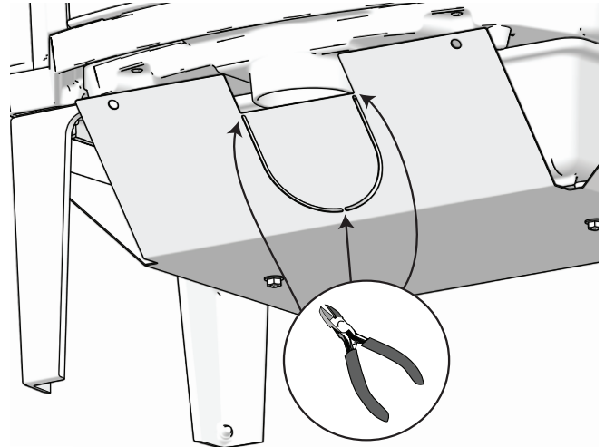
Fig. 8a Mounting of external air supply connection
