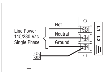
Single Phase Power Wiring
