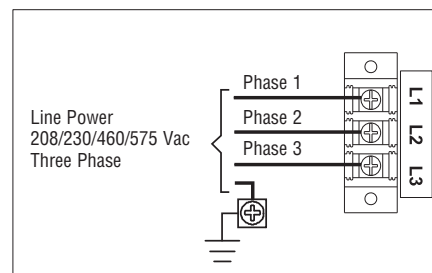
Three Phase Power Wiring
