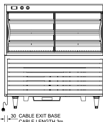
REAR ELEVATION
