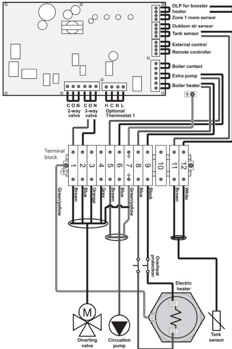
3.6.4 Electrical wiring diagram - main PCB of Heat Pump (Aquarea H and J series)
