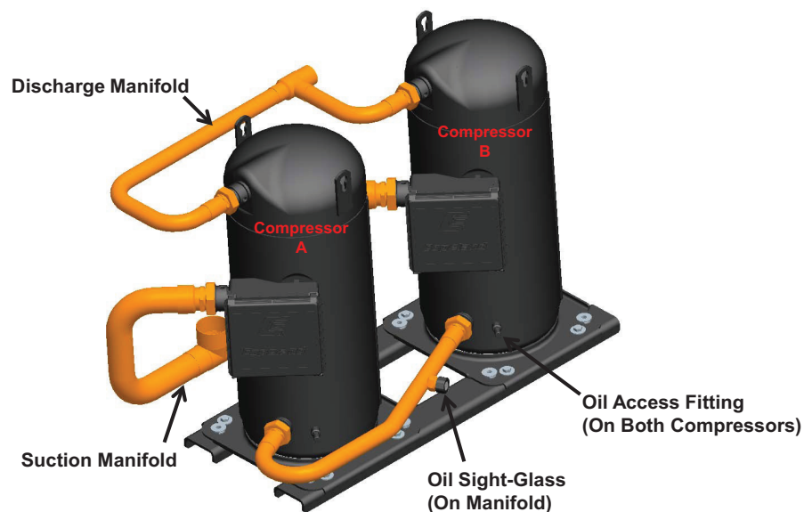
Figure 6 – Typical Rotolock Connected Tandem with TPTL Oil Manifold
