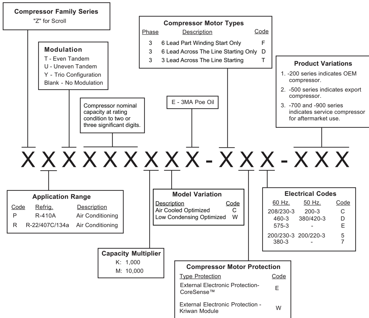
Figure 1 – Nomenclature
