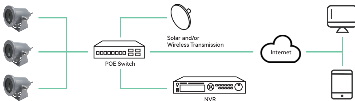
Figure 1-1 Connection diagram
