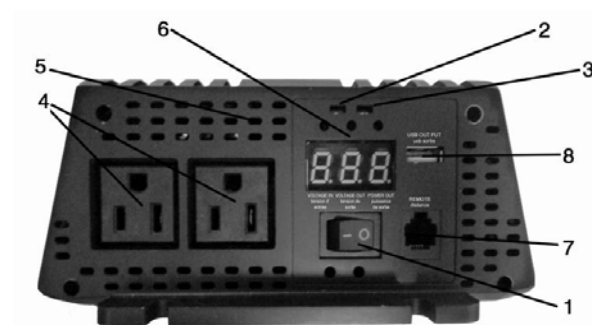
Figure 2-1 AC Panel
