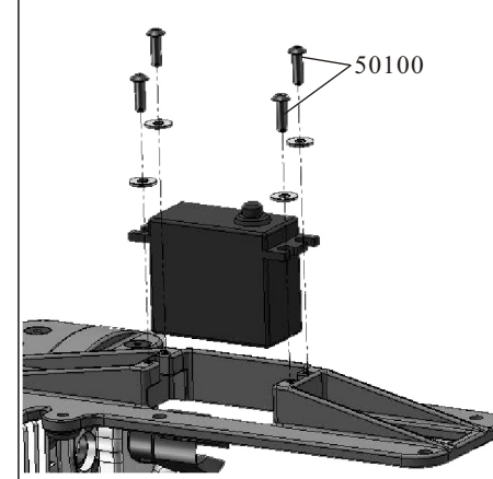
Front Brace Assembly
