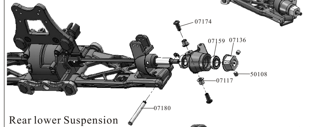
Steering Mount Assembly
