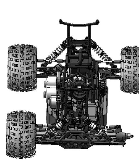
Wheels Complete Assembly
