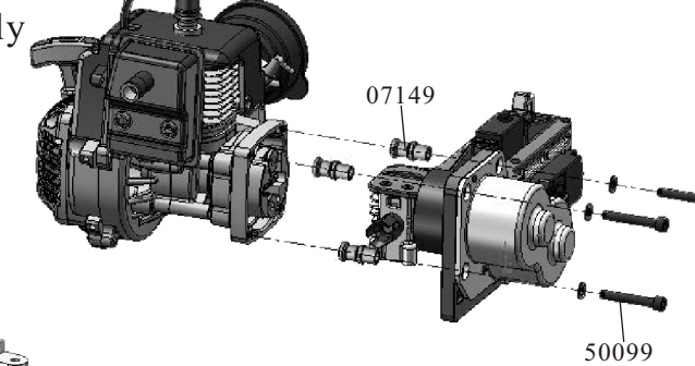
Center Unit Assembly
