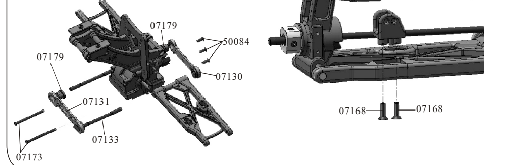
Rear lower Suspension Arms Assembly
