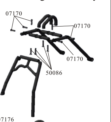
Roll Cage Assembly
