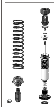
Rear Shock Absorber Exploded View(Long)
