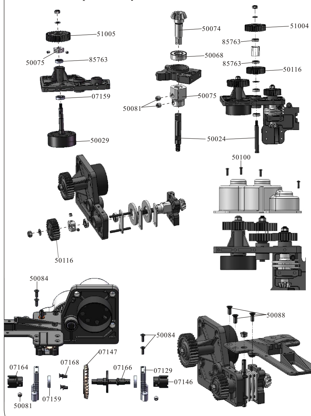
Diff.Gear Group Assembly
