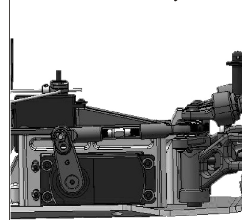
Servo link Assembly
