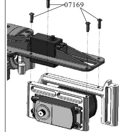
Throttle Link Assembly
