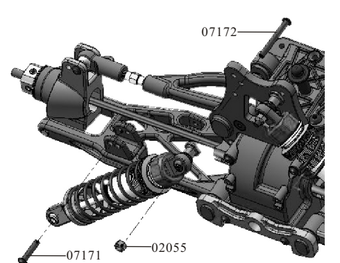
Rear Shock Absorber Assembly
