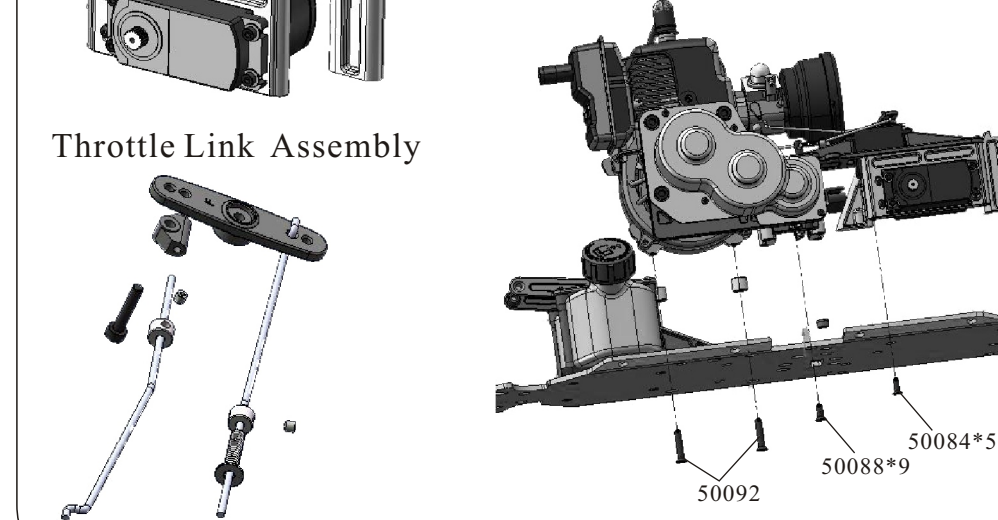
Center Unit Assembly
