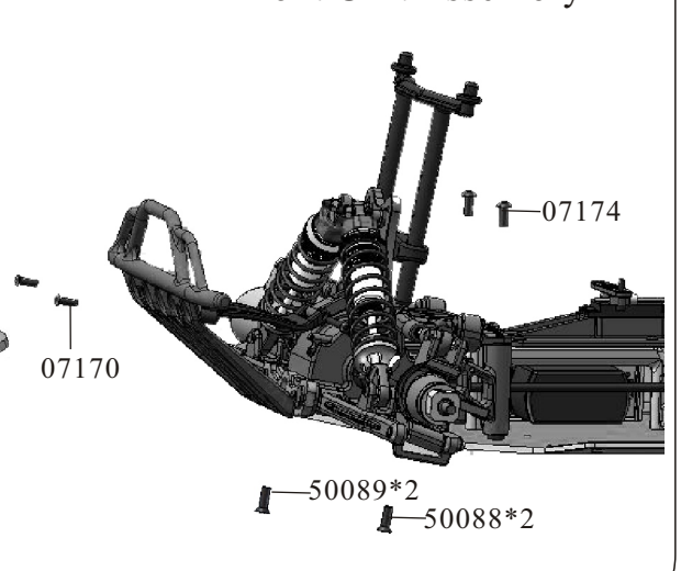
Front Unit Assembly
