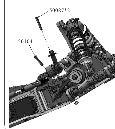
Steering link Assembly
