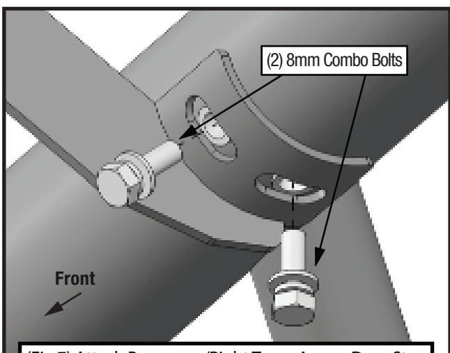
(Fig 7) Attach Passenger/Right Tyger Access Drop Step to Passenger/Right Mounting Brackets, as shown, for all mounting brackets.
