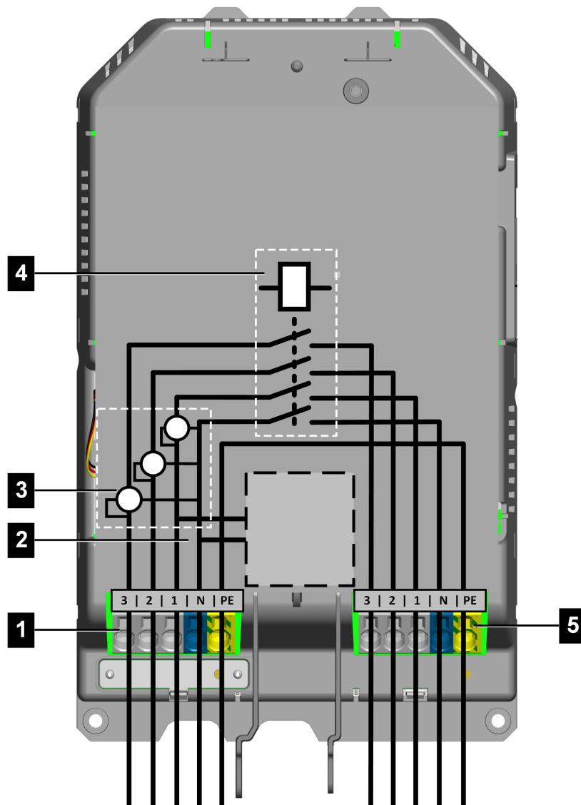
Fig. 3-3: Measurement scheme
