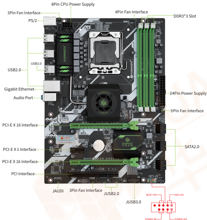
1-1 X58 DELUXE motherboard illustration
