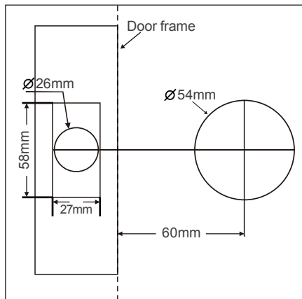
Installation Template
