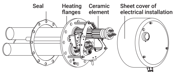
TPK – three-phase
