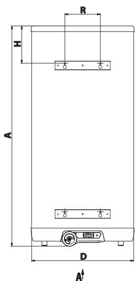
OKHE ONE 30–120
