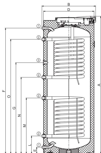
OKC 200, 250 NTRR
