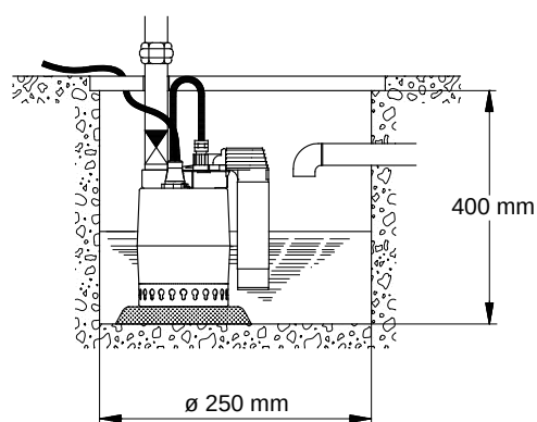
Fig. 9 Minimum well dimensions, Unilift KP-AV
