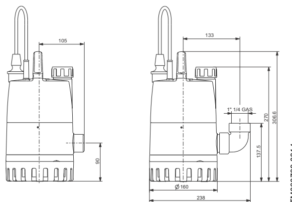
Fig. 6 Pump dimensions
