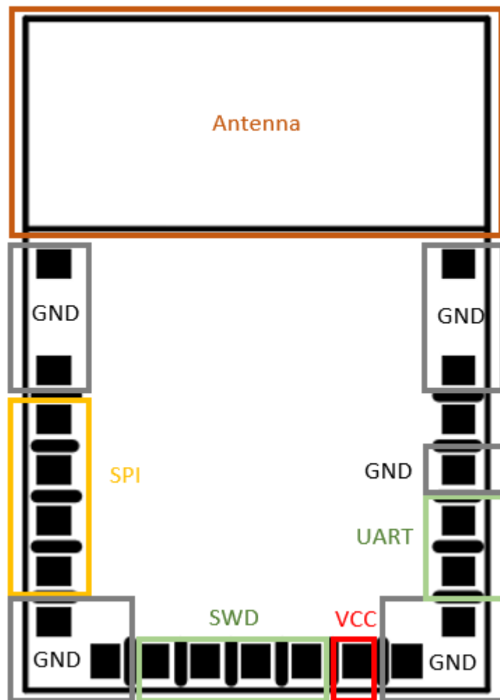
Figure 2. Solder PAD
