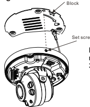
Figure 3-4 Install device
