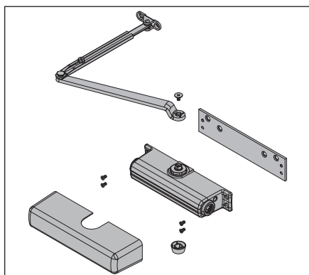
EDA &amp; CUSH Arm Assemblies
