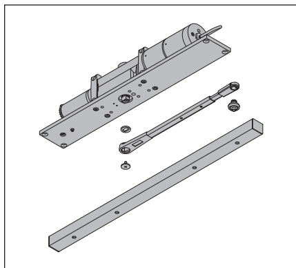
Arm &amp; Track
