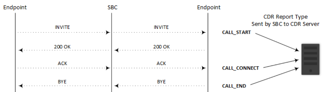
Figure 50-2: CDR Report Types for SBC Signaling
