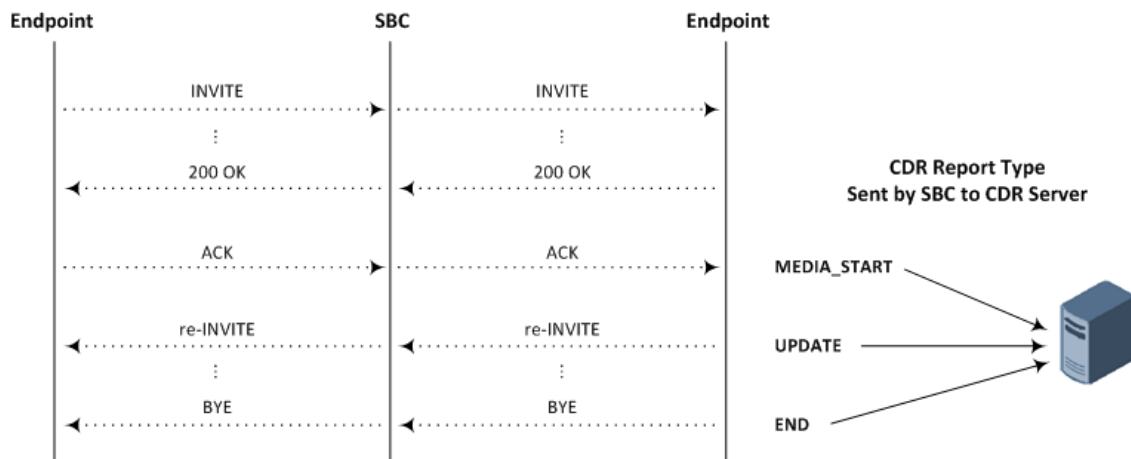
Figure 50-1: CDR Report Types for SBC Media
