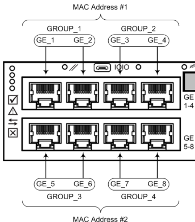
Figure 13-1: Mediant 9000 Ethernet Port String Names
