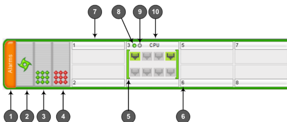
Figure 42-1: Graphical Display of Device on Monitor Page - Mediant 2600 Enterprise Session Border Controller
