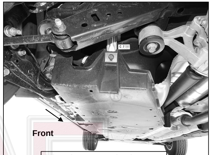
(Fig 23) Remove plastic cover
