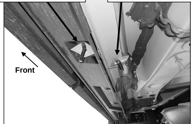
(Fig 16) Insert 8mm Bolt Plate and 10mm L-Shaped Bolt into the Passenger/Right Center mounting holes
