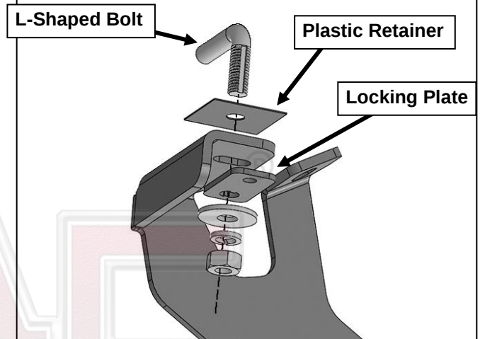
(Fig 14) L-Shaped Bolt installation
