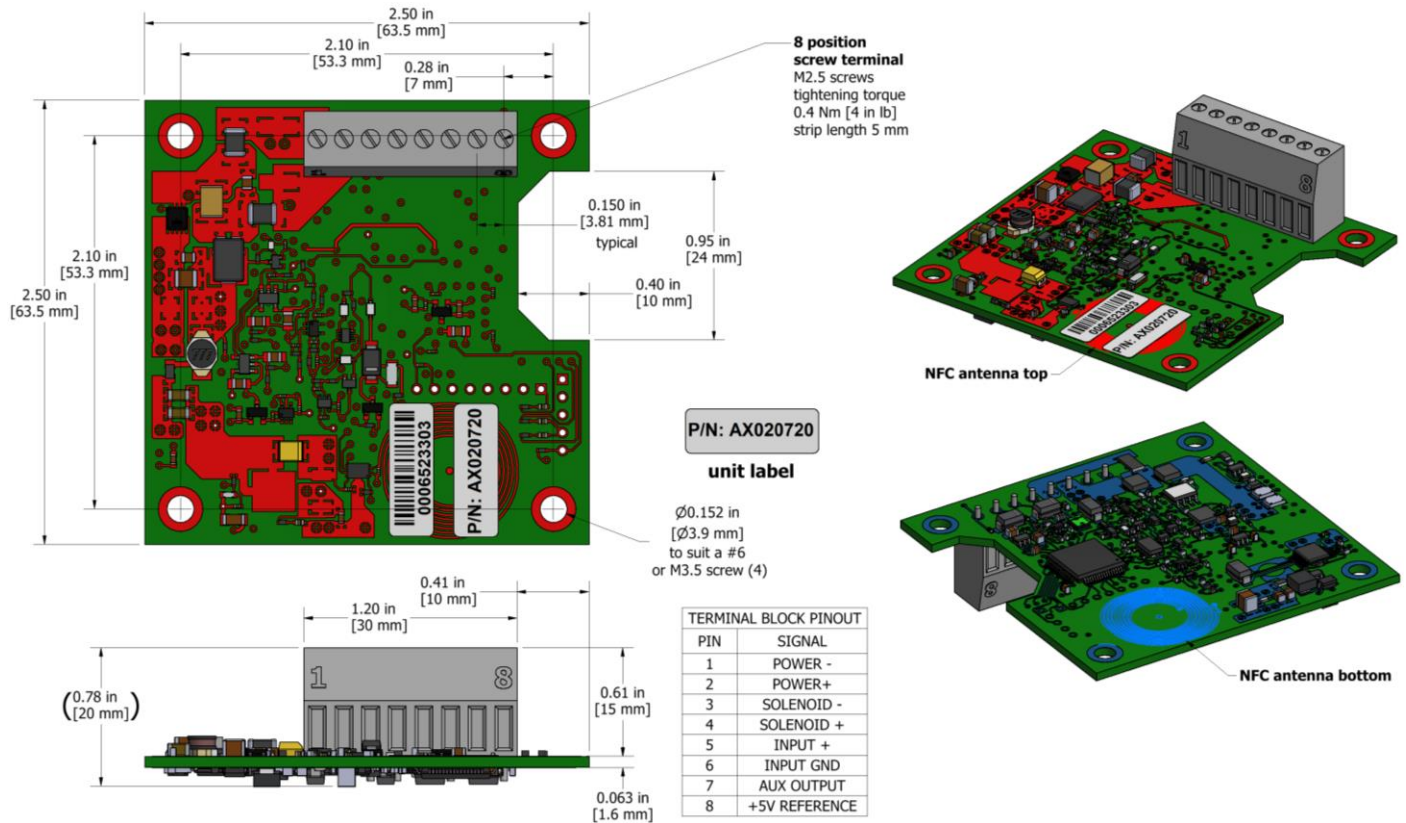
Figure 4 – Board Dimensions
