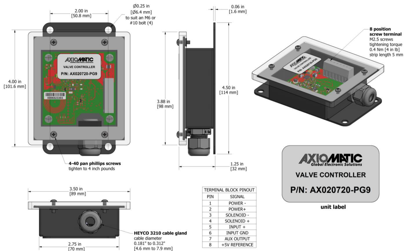
Figure 5 – Board Dimensions
