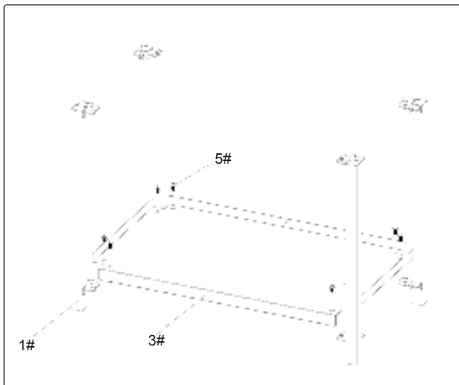
Step 1. Assemble the uprights, bottom panel with screws M6*12 as shown.
