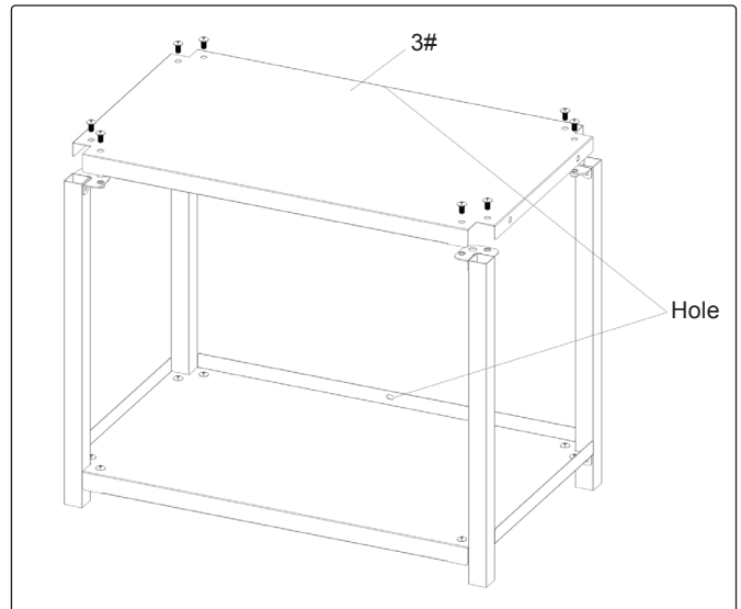
Step 2. Assemble the top panel with screws M6*12.
