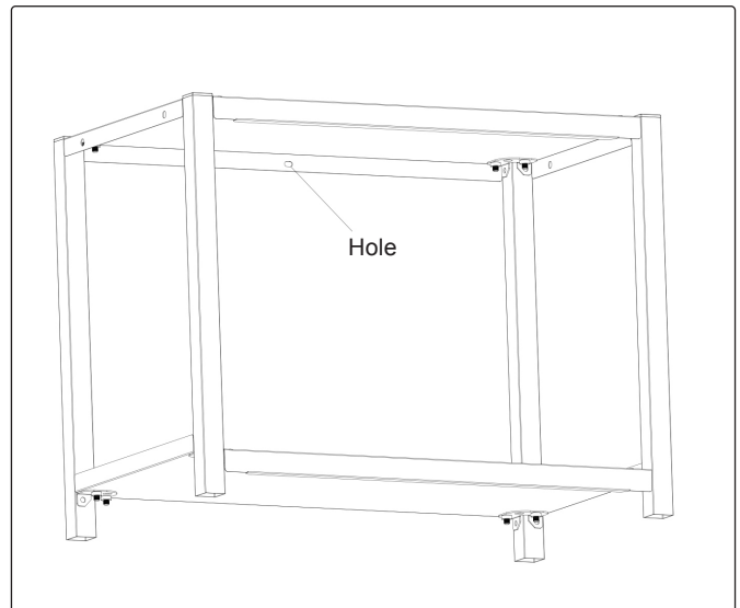
Step 4. To fix on the wall, mark the wall according to the hole which is at the back of top panel, after assembly.
