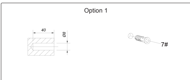
Step 5. To fix the cabinet on to the wall. Mark the wall out before drilling the hole, after the wall has been marked drill a hole the size required as illustration, Insert the wall plug 8*40.
