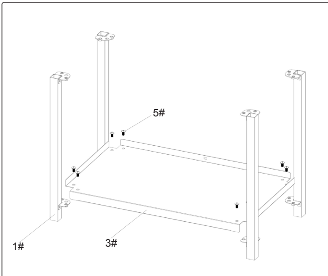
Step 1. Assemble the uprights, bottom panel with screws M6*12 as shown.
