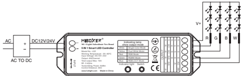
Controller connect to RGBW LED strip diagram
