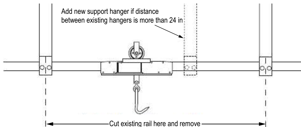
Figure 2-5. MS202 Rail Installation
