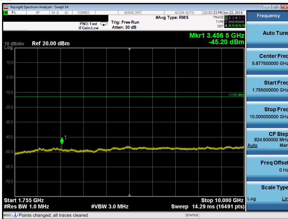
Plot 7-65. Conducted Spurious Plot (Band 4 – 10.0MHz QPSK – RB Size 1, RB Offset 0 – Mid Channel)
