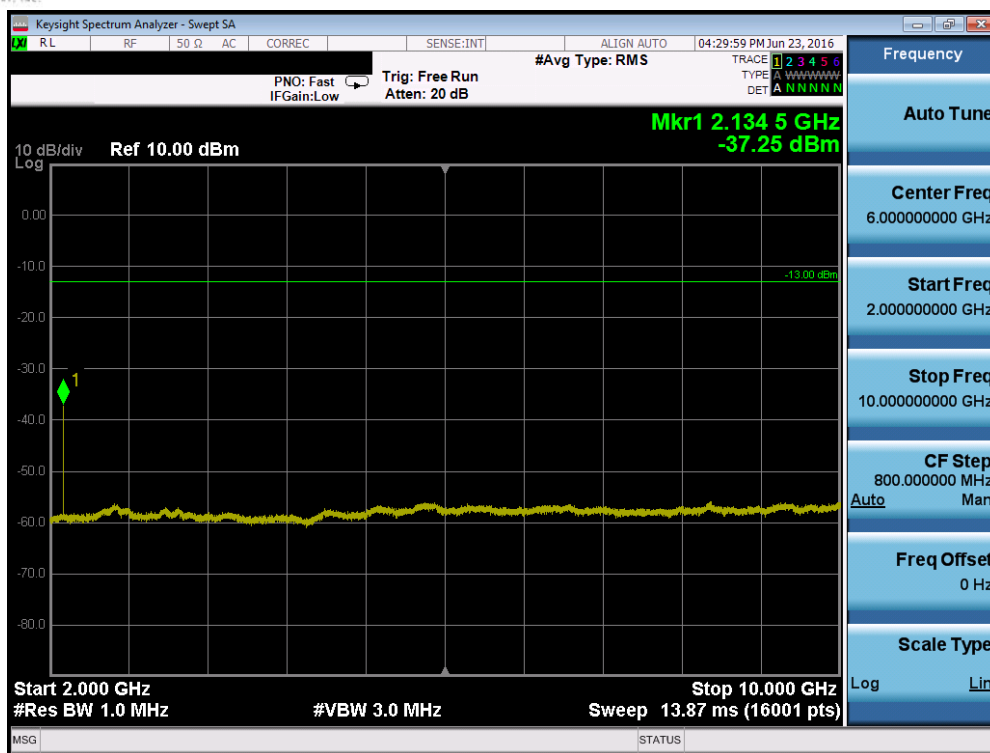
Plot 7-51. Conducted Spurious Plot (Band 12 – 5.0MHz QPSK – RB Size 1, RB Offset 0 – High Channel)
