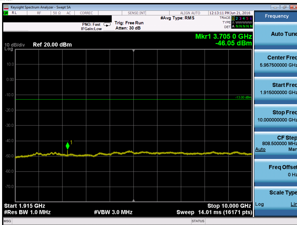
Plot 7-71. Conducted Spurious Plot (Band 2/25 – 5.0MHz QPSK – RB Size 1, RB Offset 0 – Low Channel)
