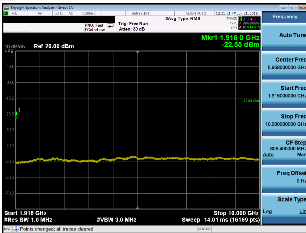
Plot 7-77. Conducted Spurious Plot (Band 2/25 – 5.0MHz QPSK – RB Size 1, RB Offset 0 – High Channel)
