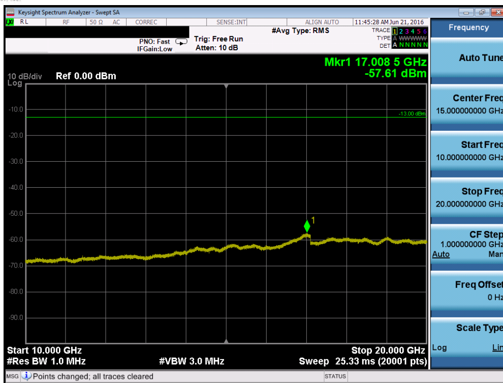
Plot 7-75. Conducted Spurious Plot (Band 2/25 – 5.0MHz QPSK – RB Size 1, RB Offset 0 – Mid Channel)
