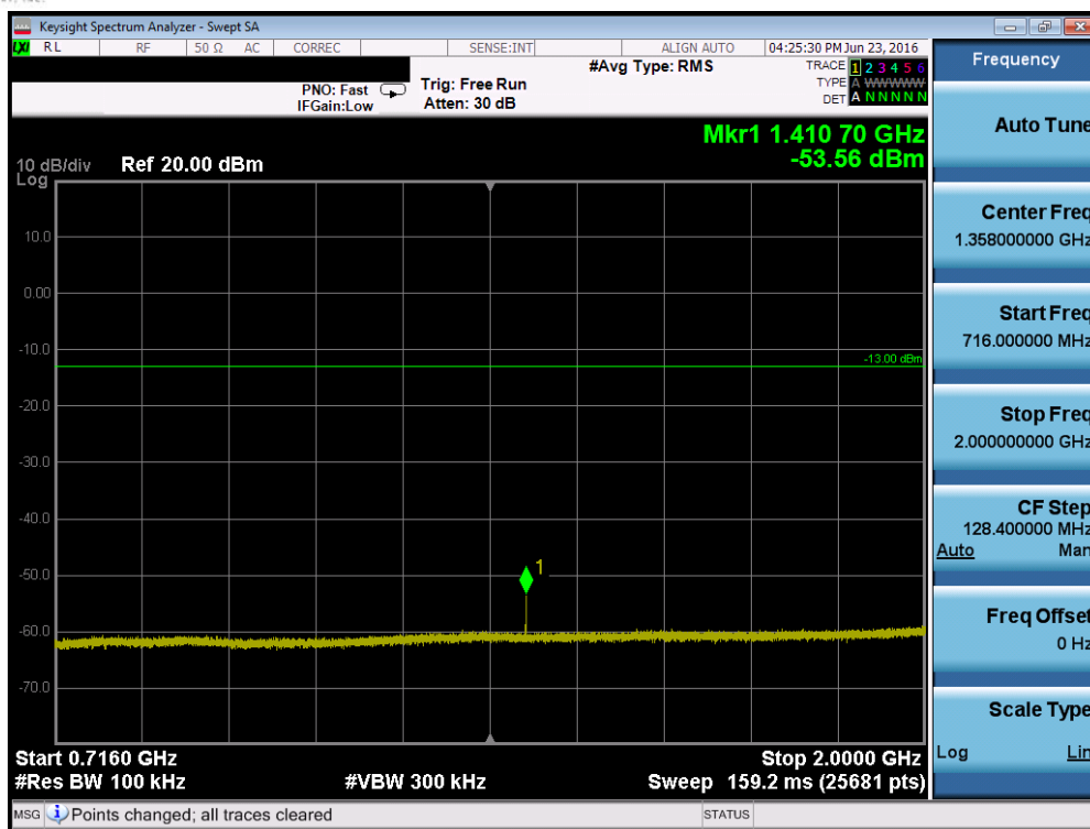
Plot 7-47. Conducted Spurious Plot (Band 12 – 5.0MHz QPSK – RB Size 1, RB Offset 0 – Mid Channel)
