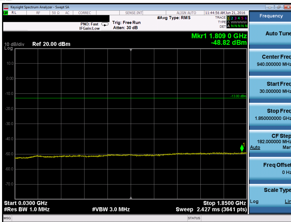
Plot 7-73. Conducted Spurious Plot (Band 2/25 – 5.0MHz QPSK – RB Size 1, RB Offset 0 – Mid Channel)
