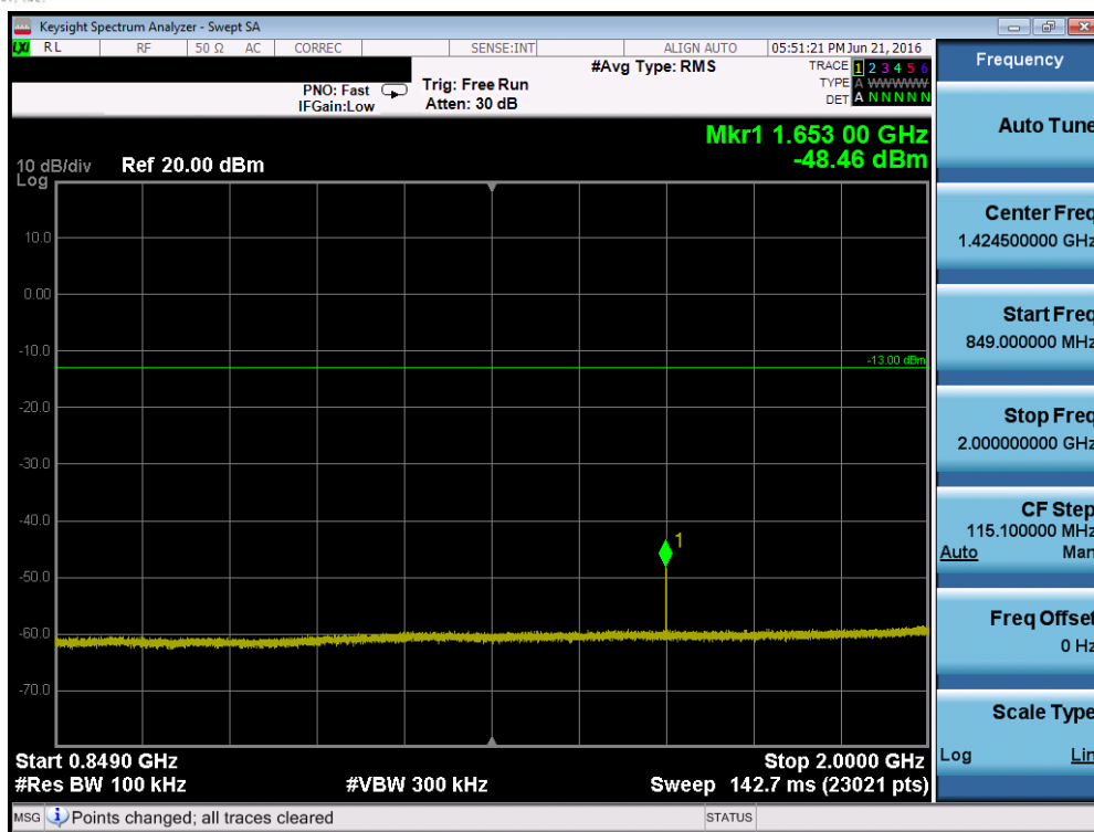
Plot 7-53. Conducted Spurious Plot (Band 5/26 – 5.0MHz QPSK – RB Size 1, RB Offset 0 – Low Channel)
