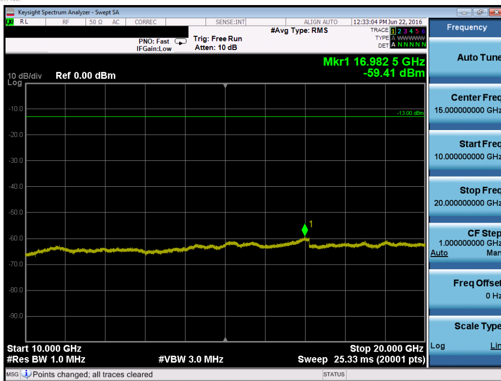
Plot 7-63. Conducted Spurious Plot (Band 4 – 10.0MHz QPSK – RB Size 1, RB Offset 0 – Low Channel)
