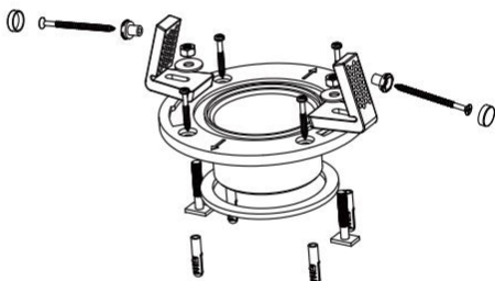
Flange, EVA Ring, Mounting Accessory Kit
