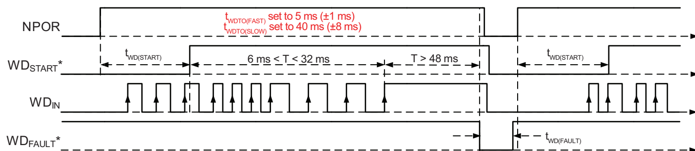
Figure 8: Window Watchdog Timer SLOW Fault, T = WD_{IN} period
