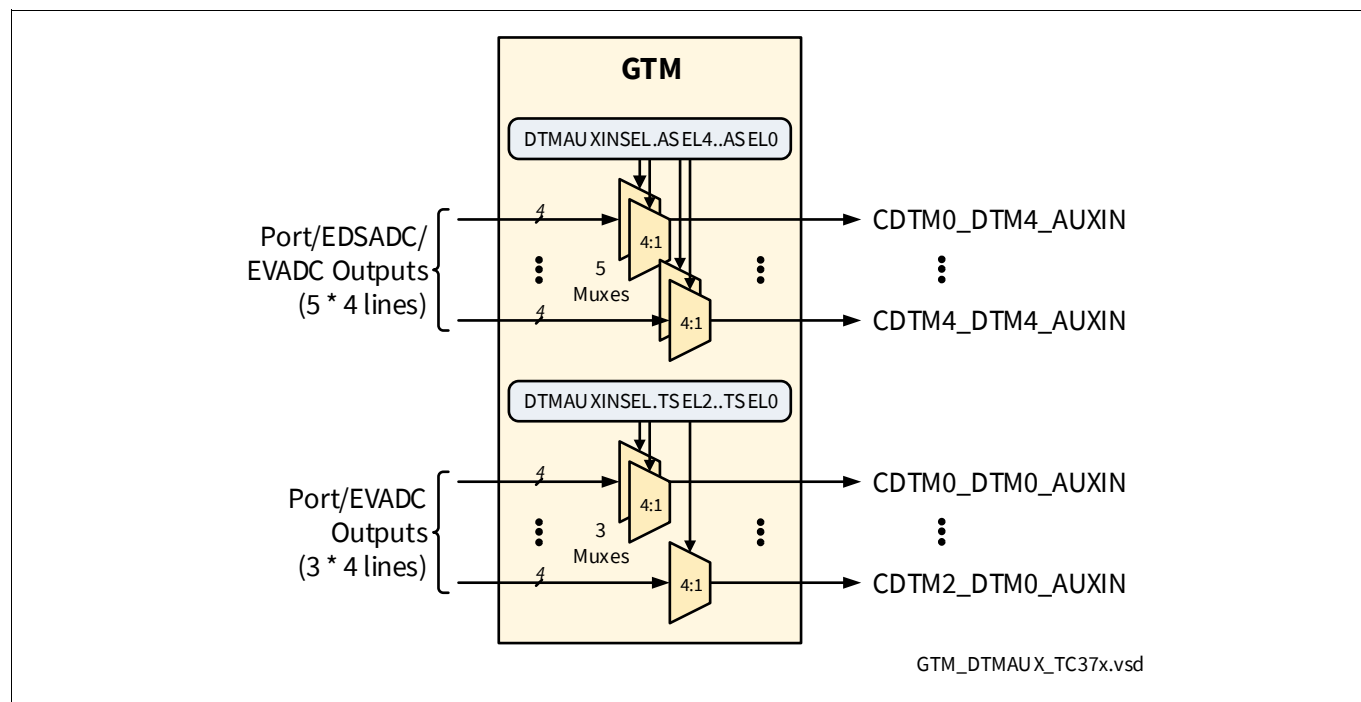
Figure 12 DTM_AUXIN Connections Overview
