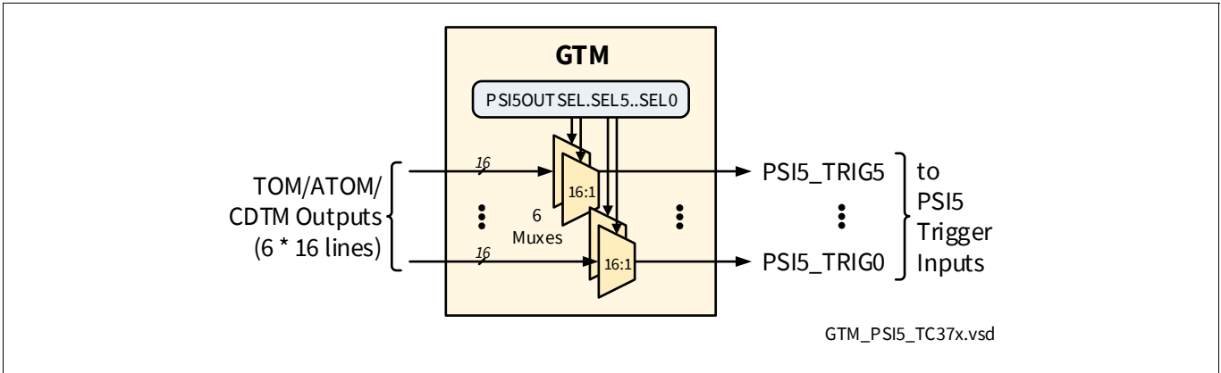
Figure 26 GTM to PSI5 Connections Overview
