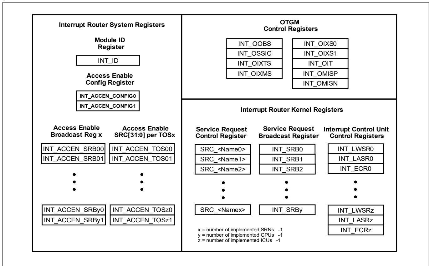
Figure 6 Interrupt Router module registers (SRC registers are described in Chapter 16.4 )
