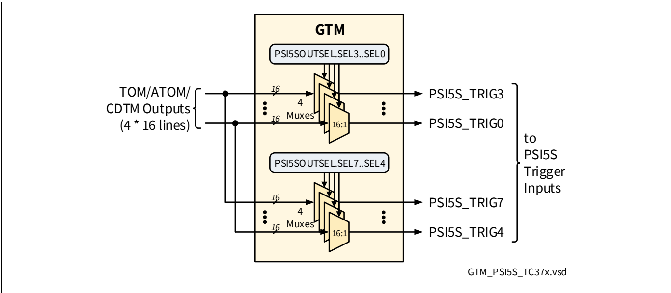
Figure 27 GTM to PSI5S Connections Overview
