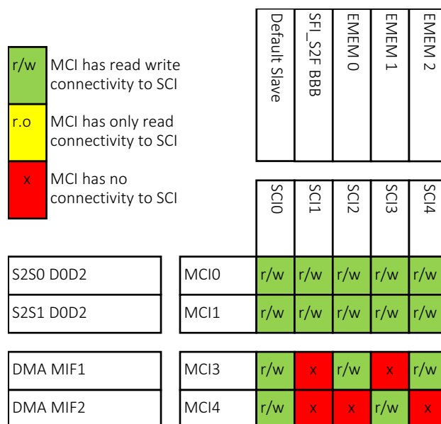
Figure 2 TC37xEXT Domain 2 Connectivity Matrix
