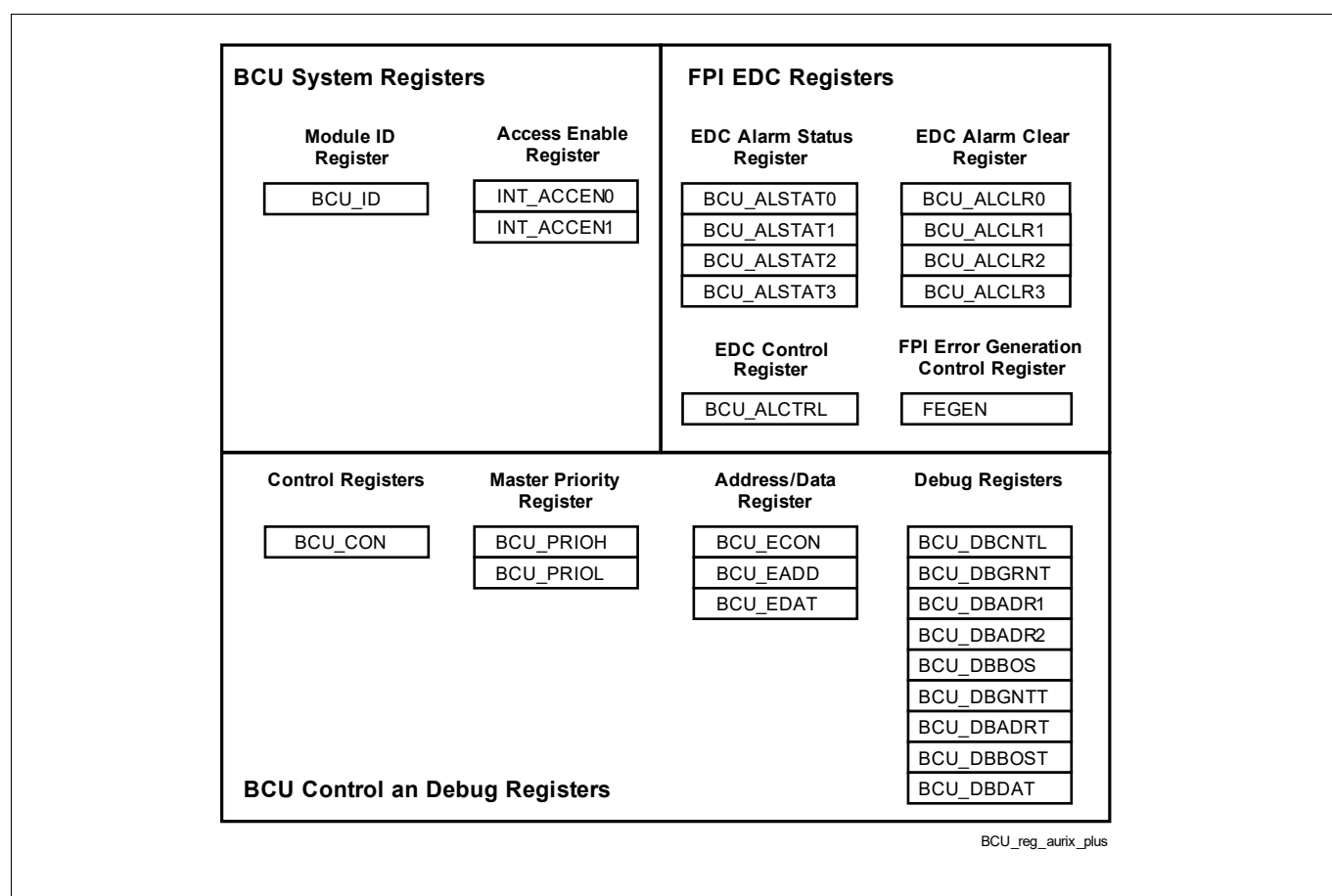
Figure 4 EBCU Registers
