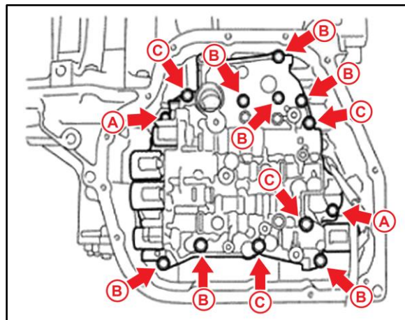
Figure 8. Transmission Valve Body
