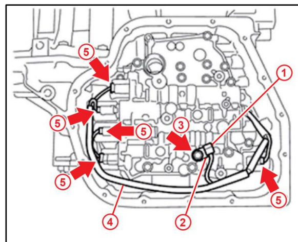
Figure 4. Transmission Valve Body Assembly
