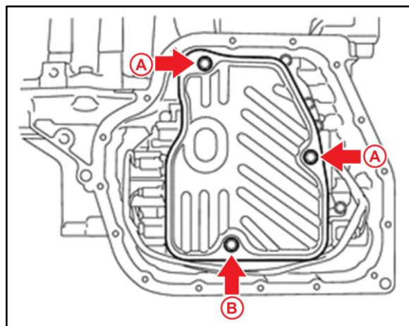
Figure 2. Oil Strainer
