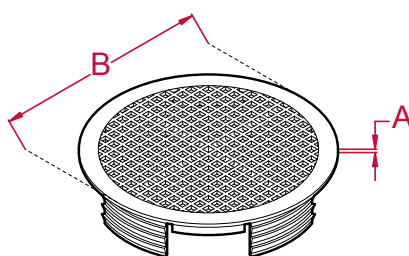
AVP70 70mm Vent Plug A: 1.75mm B: 80mm Drill hole size = 70mm
