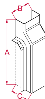
AK105T15 (15mm) Skirting Cover T Connector A: 150mm B: 62mm C: 85mm
