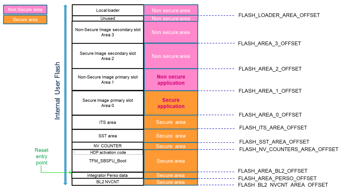
Figure 3. Flash layout
