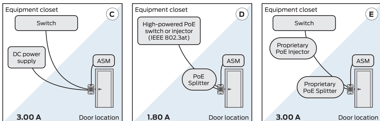
Figure 4.1: Power options
