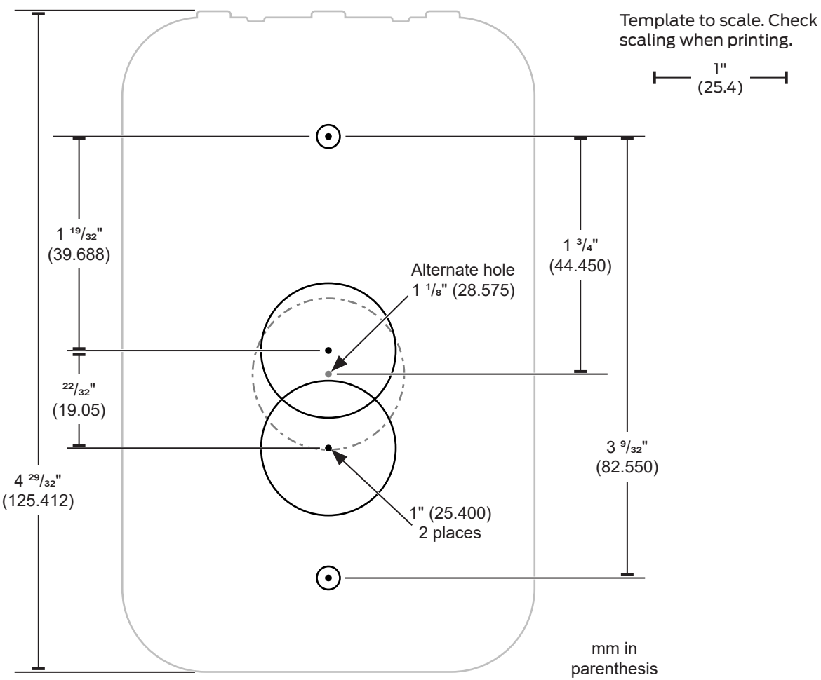
Figure 1.2: RC15/RCK15 Mounting
