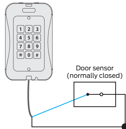
Figure 2.5: Door sensor wiring
