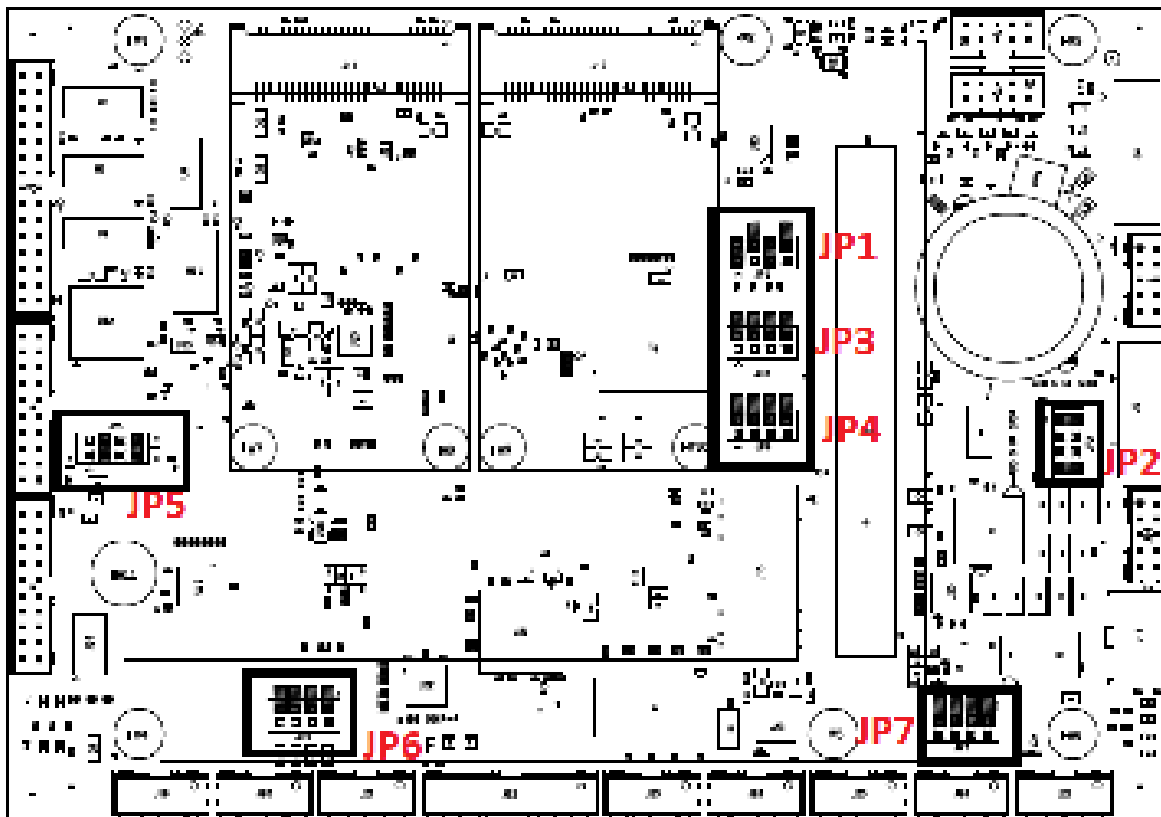
Figure 4: Jumper Blocks on Jasper Carrier Board
