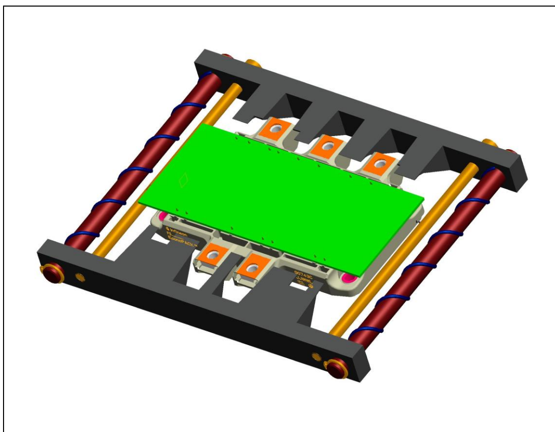
Figure 6 Exemplary press-out tool for EconoPACK™ 4 and EconoBRIDGE™ 4
