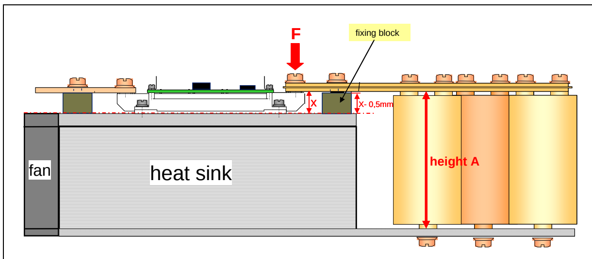
Figure 11 Concept drawing 1 of EconoPACK™ 4 assembly with ideal strain relief
