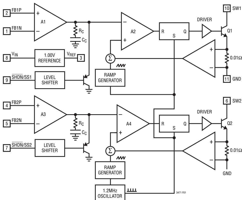
Figure 1. Block Diagram
