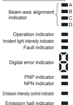
Indicator section of receiver
