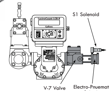
Single Stage Electro-Pneumatic Valve with V-7 Valve
