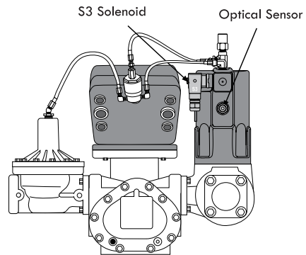
Meter System with Optical Vapor Eliminator
