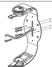
Figure 3: Pass Wire Through Hole and Attach Bracket
