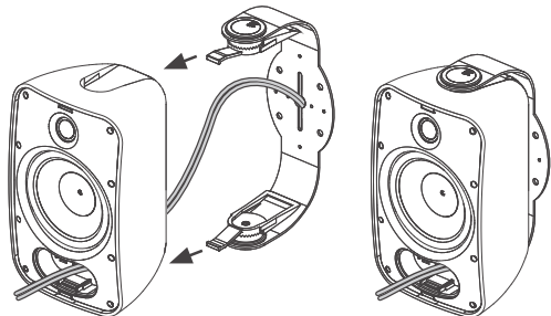
Figure 7: Attach Speakers to Brackets
