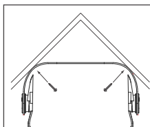
Figure 4: Corner Mounting
