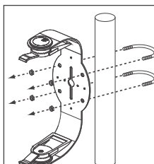
Figure 5: Attaching the Bracket to a Pole
