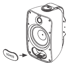
Figure 9: Attach the Connector Cover
