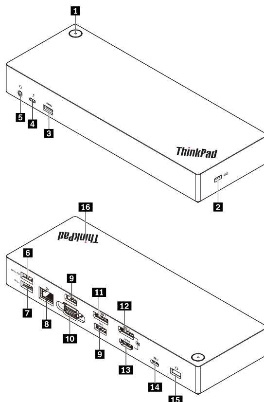
Figure 1. Dock controls, connectors, and indicators
