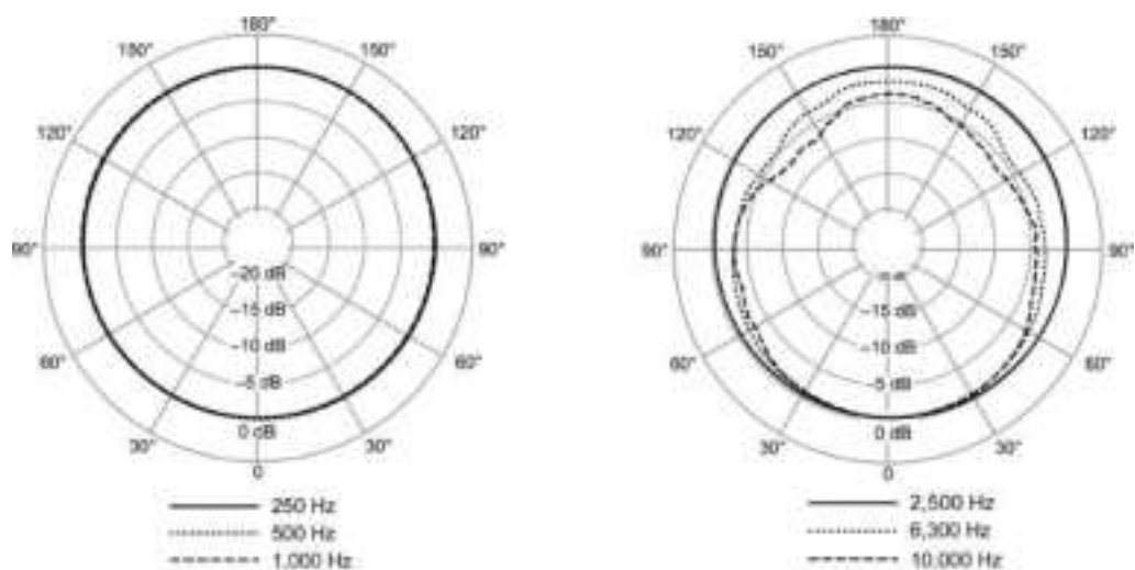
WL183m Polar Pattern
