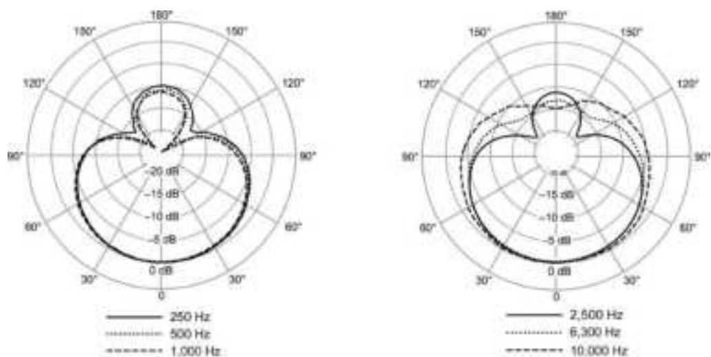
WL184m Polar Pattern
