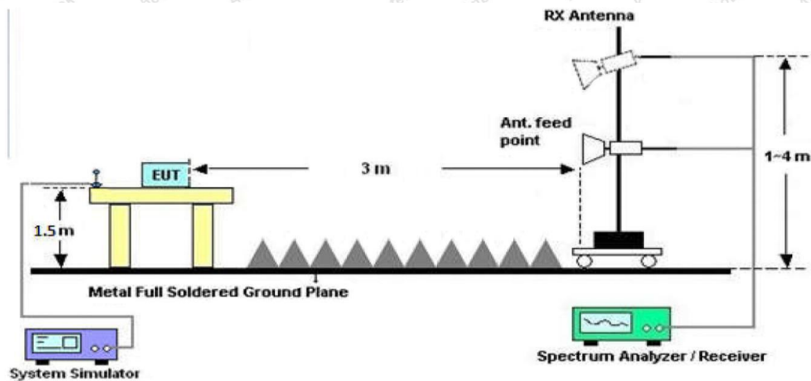
Figure 3. Above 1 GHz
