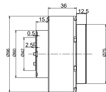
(Undriven state)
