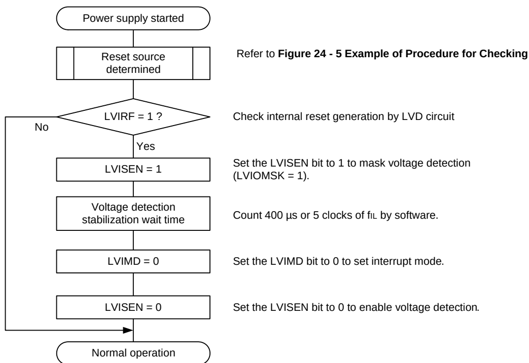
Figure 26 - 11 Setting Procedure for Initial Setting of Interrupt and Reset Mode
