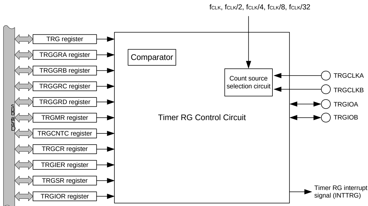
Figure 8 - 1 Timer RG Block Diagram
