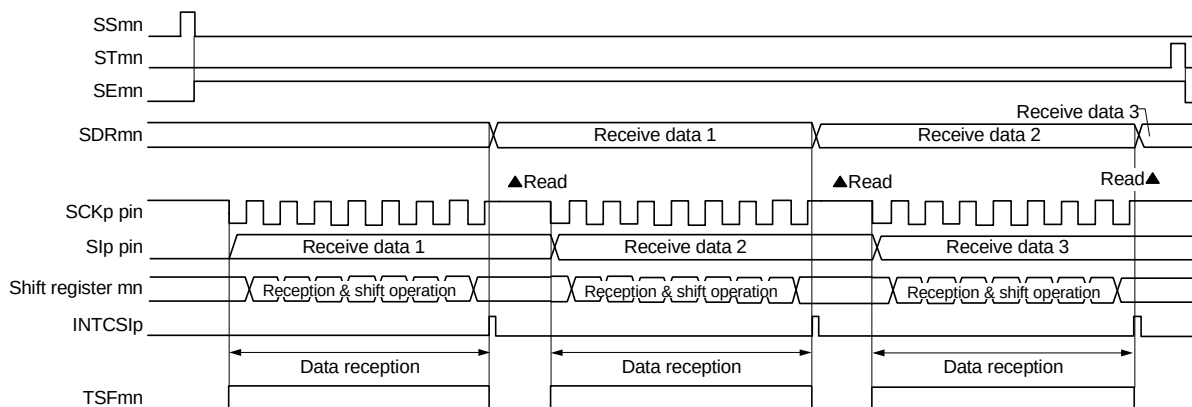
Figure 19 - 62 Timing Chart of Slave Reception (in Single-Reception Mode)
