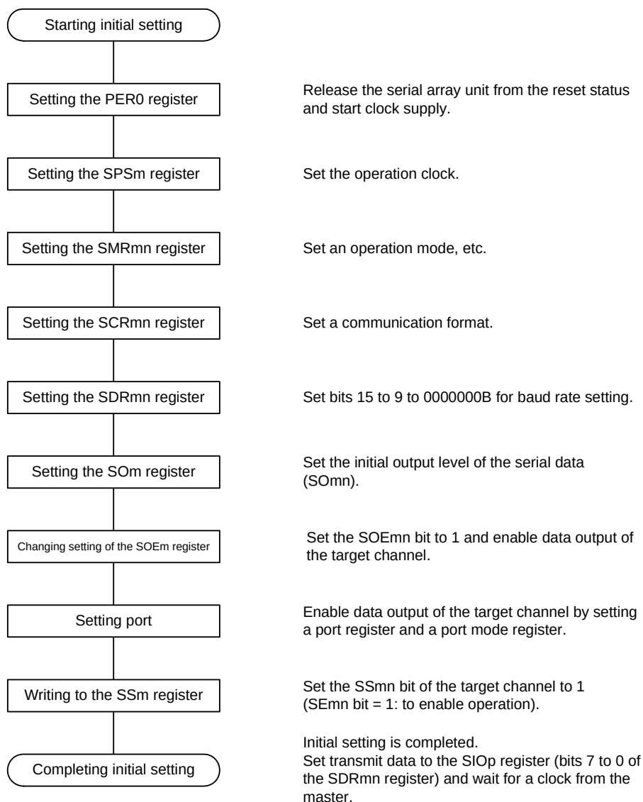
Figure 19 - 51 Initial Setting Procedure for Slave Transmission
