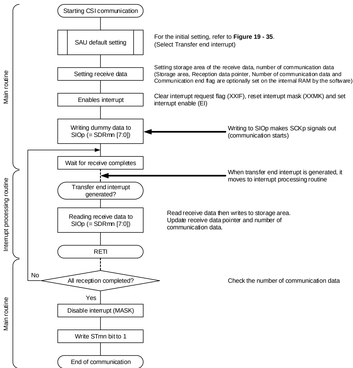
Figure 19 - 39 Flowchart of Master Reception (in Single-Reception Mode)
