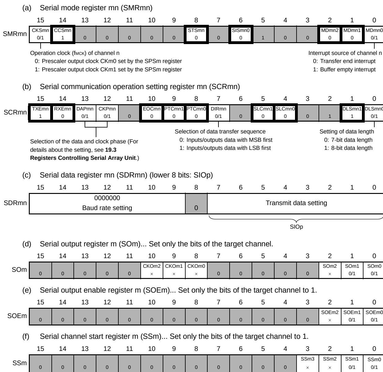
Figure 19 - 50 Example of Contents of Registers for Slave Transmission of 3-Wire Serial I/O (CSI00, CSI01)
