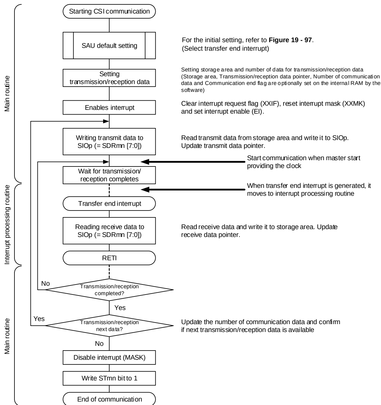
Figure 19 - 101 Flowchart of Slave Transmission/Reception (in Single- Transmission/Reception Mode)
