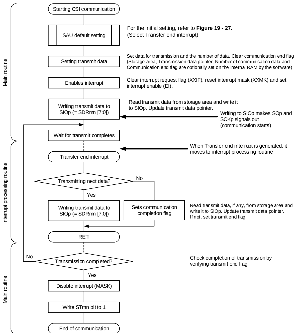
Figure 19 - 31 Flowchart of Master Transmission (in Single-Transmission Mode)
