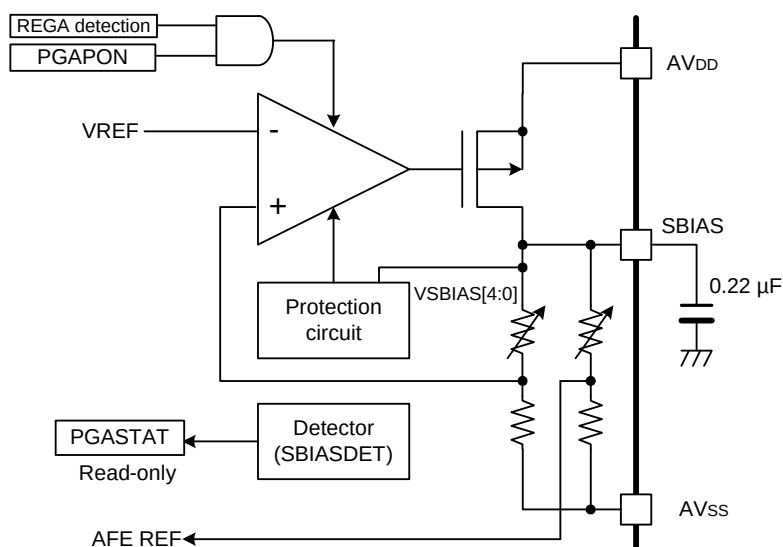
Figure 13 - 7 Block Diagram of Sensor Power Supply (SBIAS)
