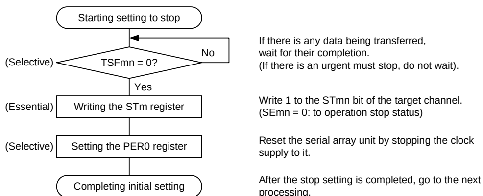
Figure 19 - 117 Procedure for Stopping UART Reception
