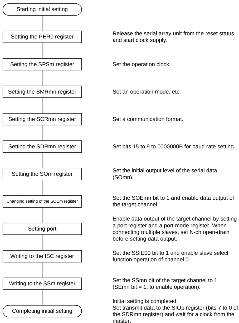
Figure 19 - 81 Initial Setting Procedure for Slave Transmission
