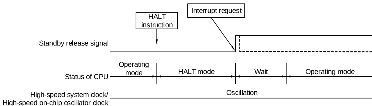
Figure 23 - 1 HALT Mode Release by Interrupt Request Generation
