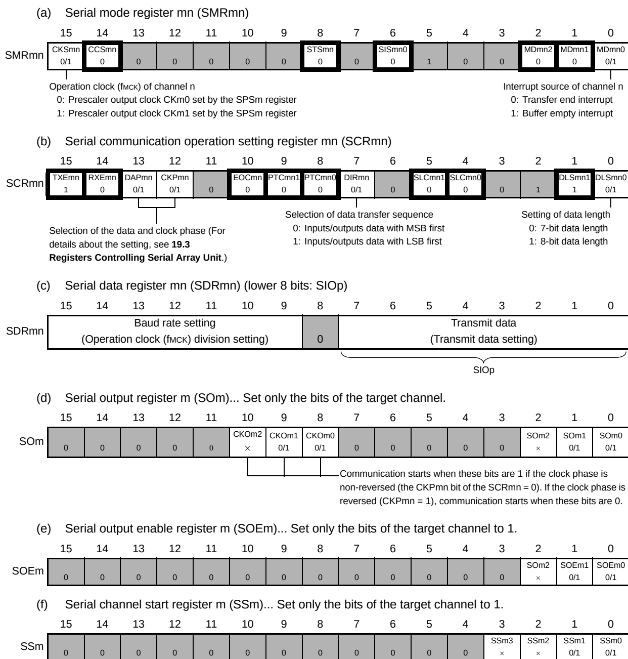
Figure 19 - 26 Example of Contents of Registers for Master Transmission of 3-Wire Serial I/O (CSI00, CSI01)
