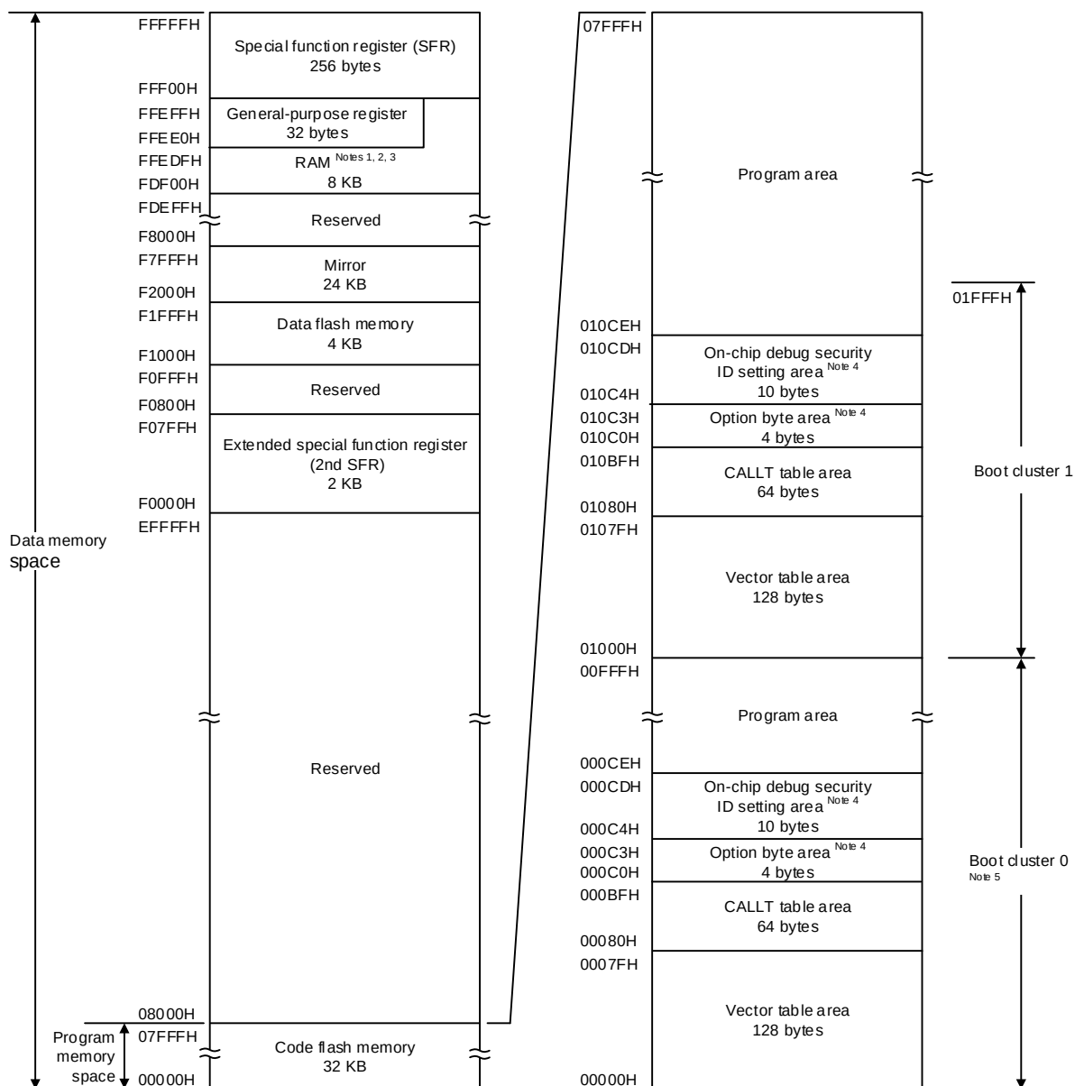
Figure 3 - 1 Memory Map (R5F11Cx (x = B, C))
