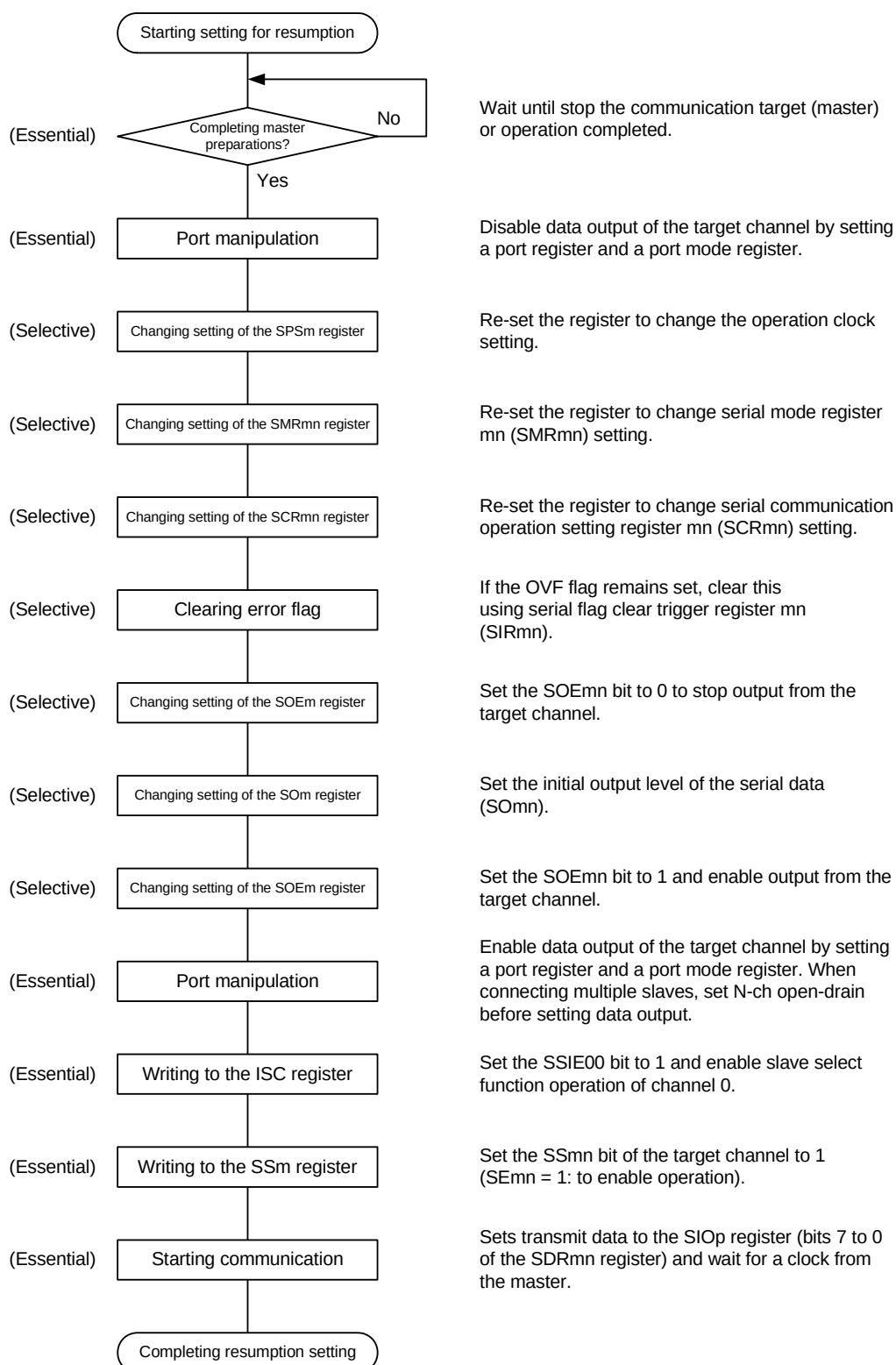
Figure 19 - 99 Procedure for Resuming Slave Transmission/Reception
