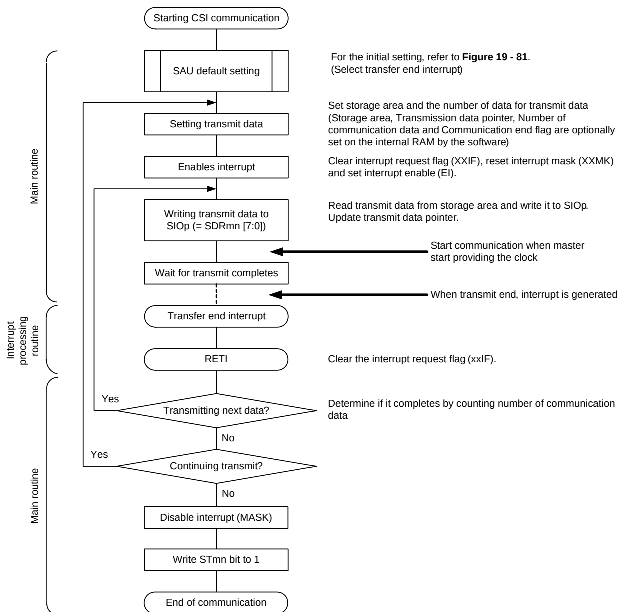
Figure 19 - 85 Flowchart of Slave Transmission (in Single-Transmission Mode)
