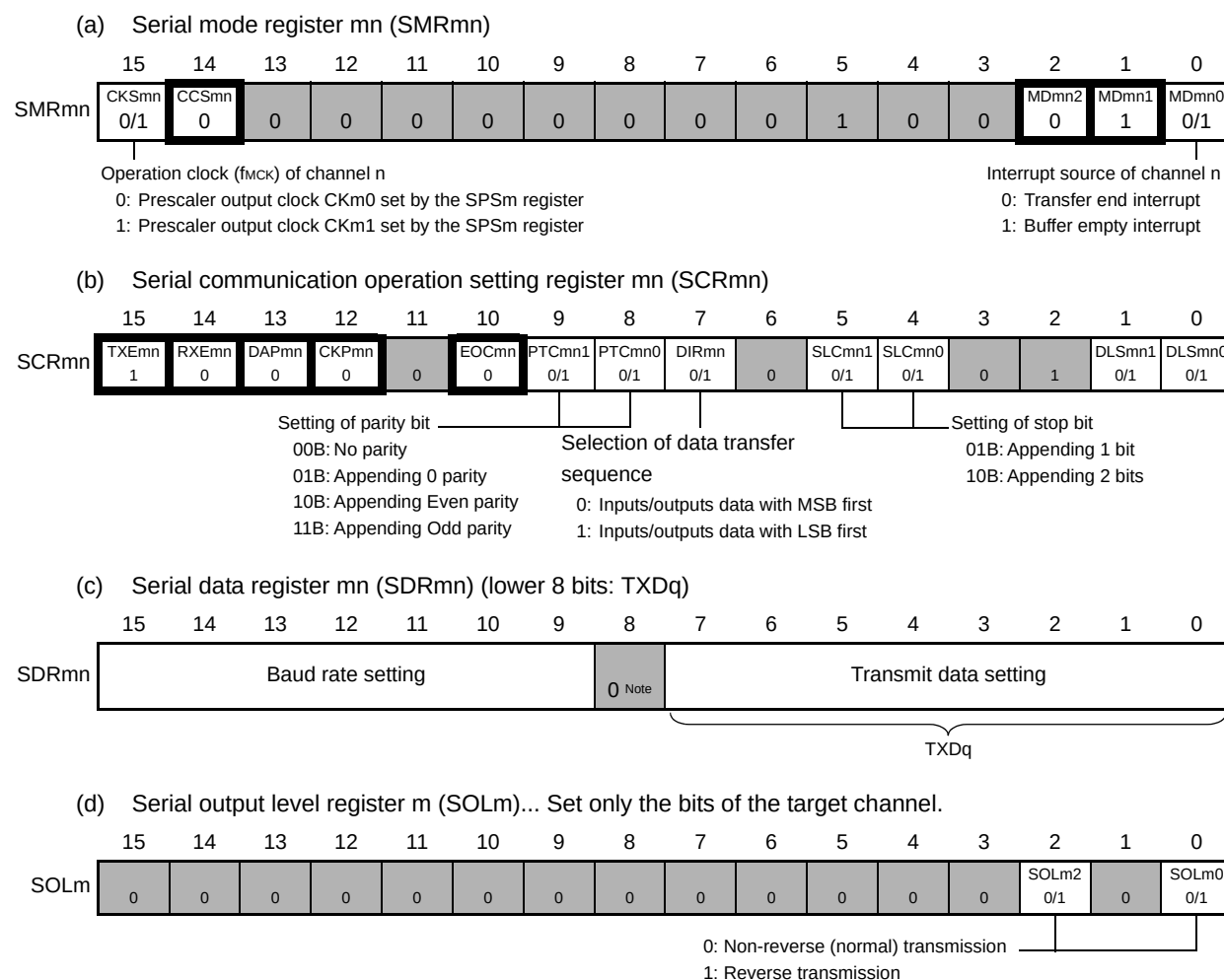
Figure 19 - 105 Example of Contents of Registers for UART Transmission of UART (UART0, UART1) (1/2)
