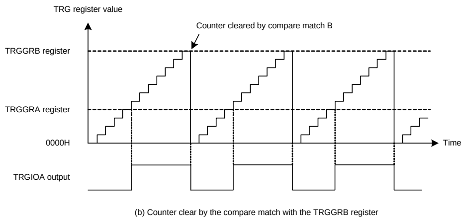
(b) Counter clear by the compare match with the TRGGRB register
