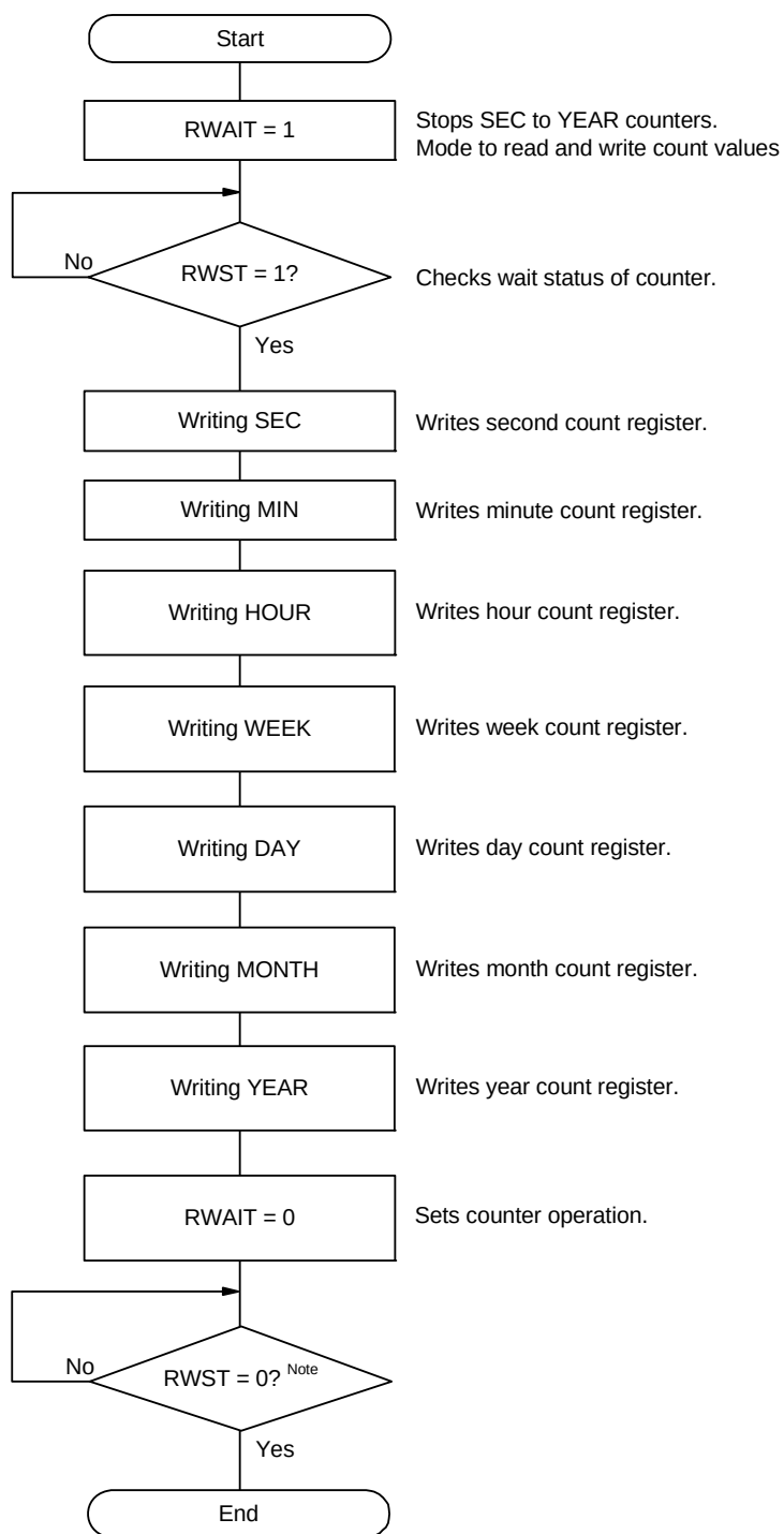
Figure 9 - 25 Procedure for Writing Real-time Clock
