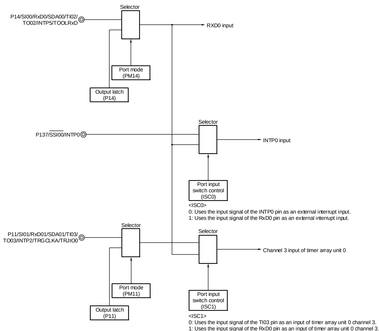
Figure 19 - 133 Port Configuration for Manipulating Reception of LIN
