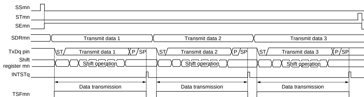
Figure 19 - 110 Timing Chart of UART Transmission (in Single-Transmission Mode)
