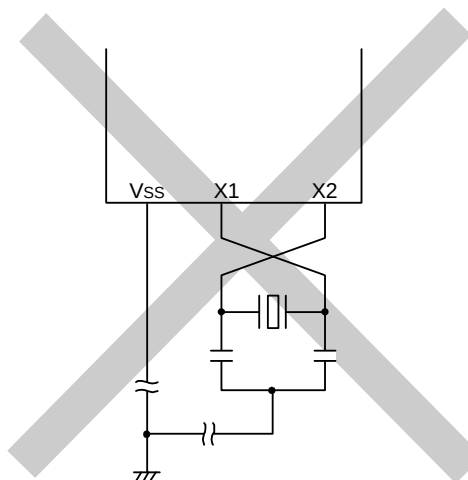
(c) The X1 and X2 signal line wires cross.
