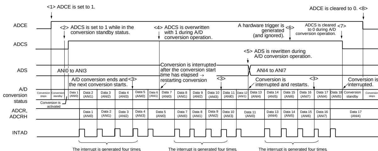
Figure 16 - 21 Example of Software Trigger Mode (Scan Mode, Sequential Conversion Mode) Operation Timing
