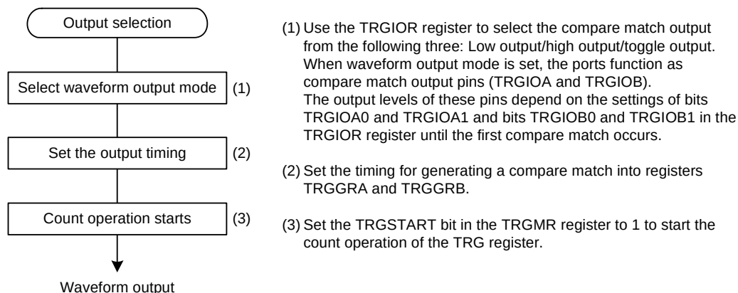
Figure 8 - 19 Procedure Example for Setting Waveform Output by Compare Match
