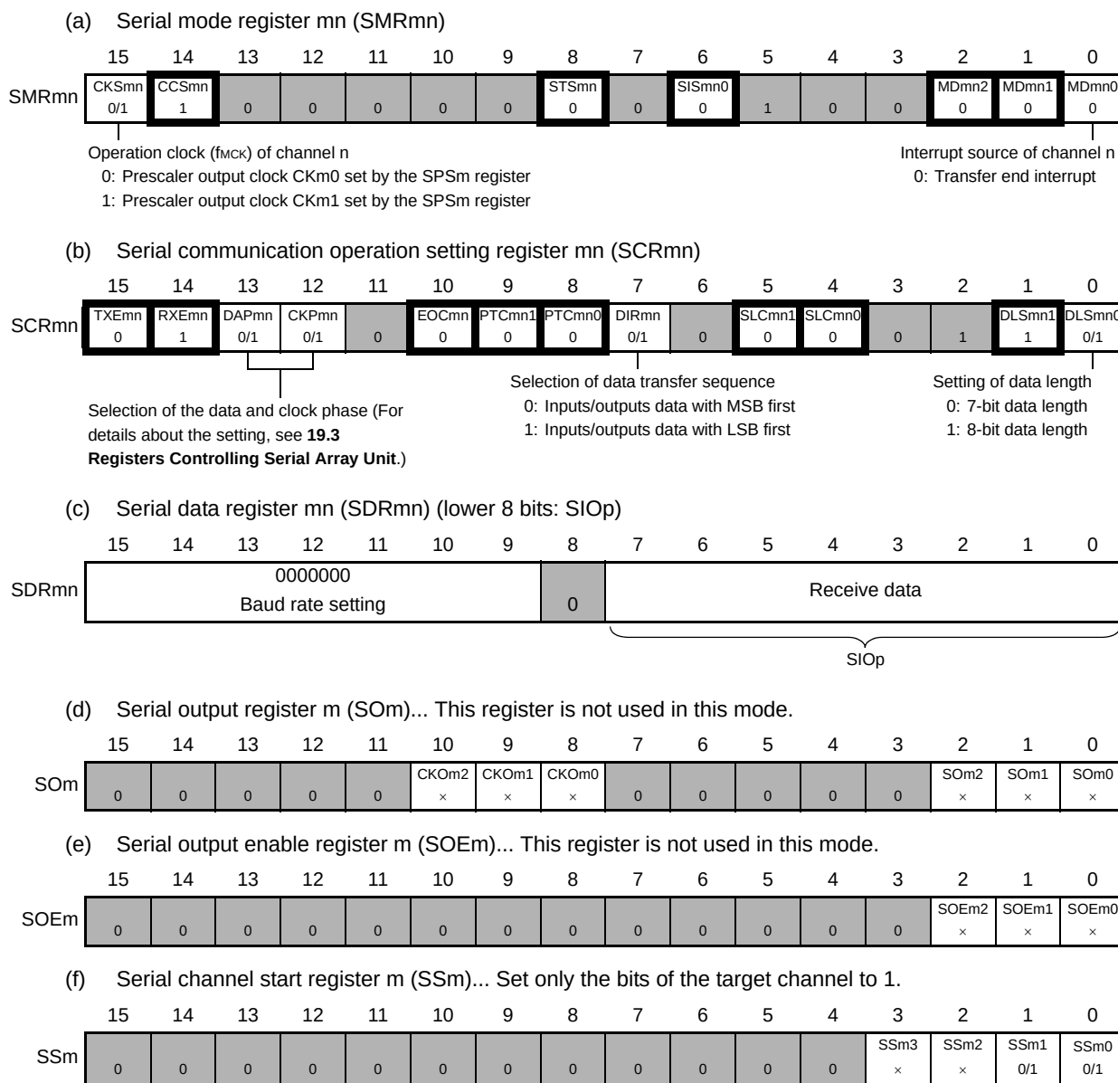
Figure 19 - 58 Example of Contents of Registers for Slave Reception of 3-Wire Serial I/O (CSI00, CSI01)
