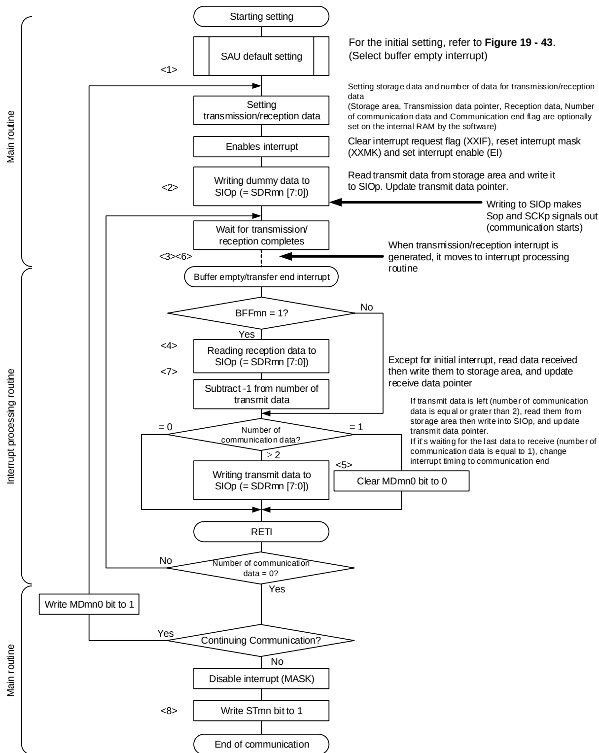
Figure 19 - 49 Flowchart of Master Transmission/Reception (in Continuous Transmission/Reception Mode)
