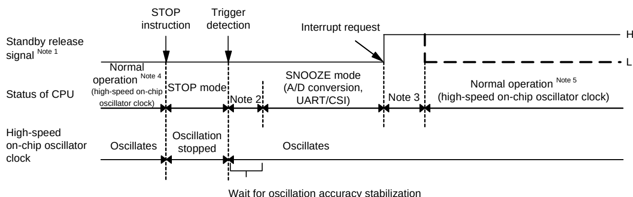
Figure 23 - 6 When the Interrupt Request Signal is Generated in the SNOOZE Mode
