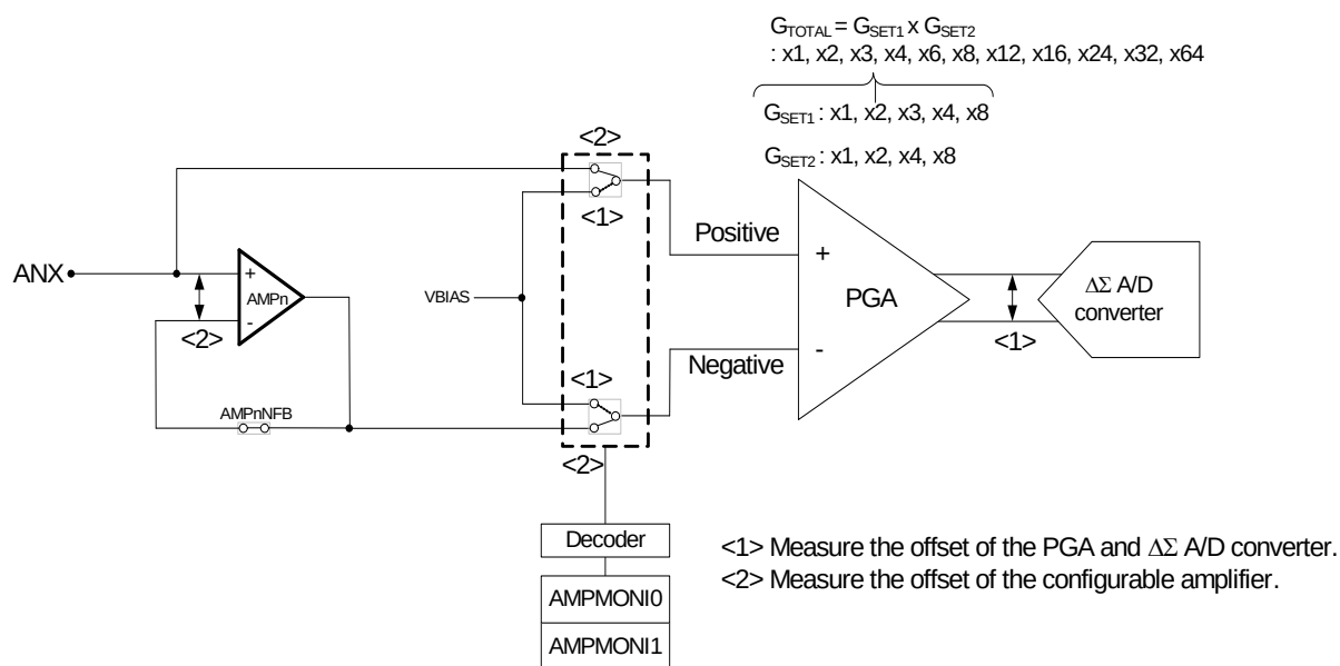
Figure 17 - 29 Offset Trimming Circuit Configuration
