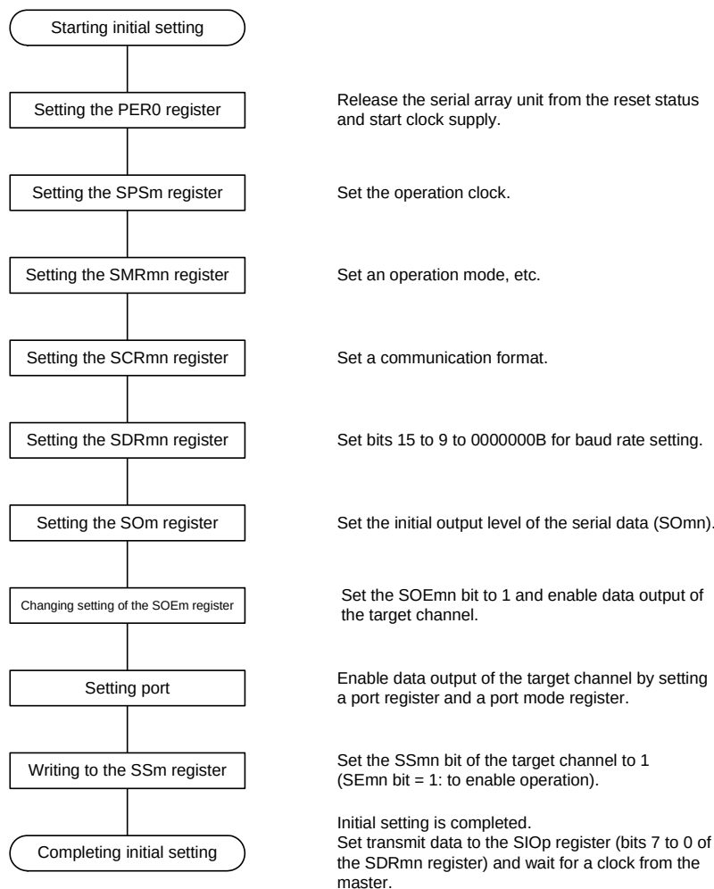
Figure 19 - 65 Initial Setting Procedure for Slave Transmission/Reception
