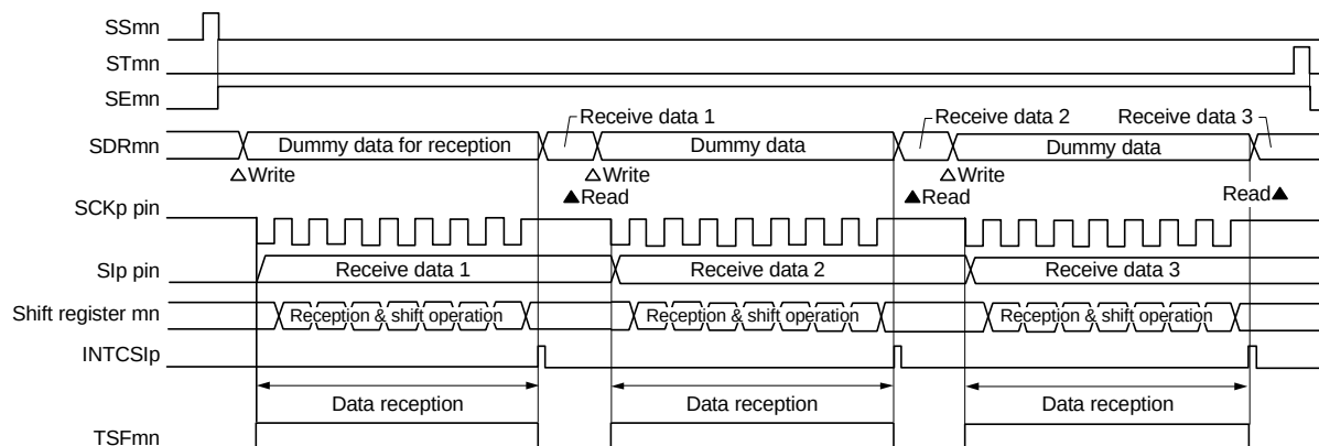
Figure 19 - 38 Timing Chart of Master Reception (in Single-Reception Mode)
