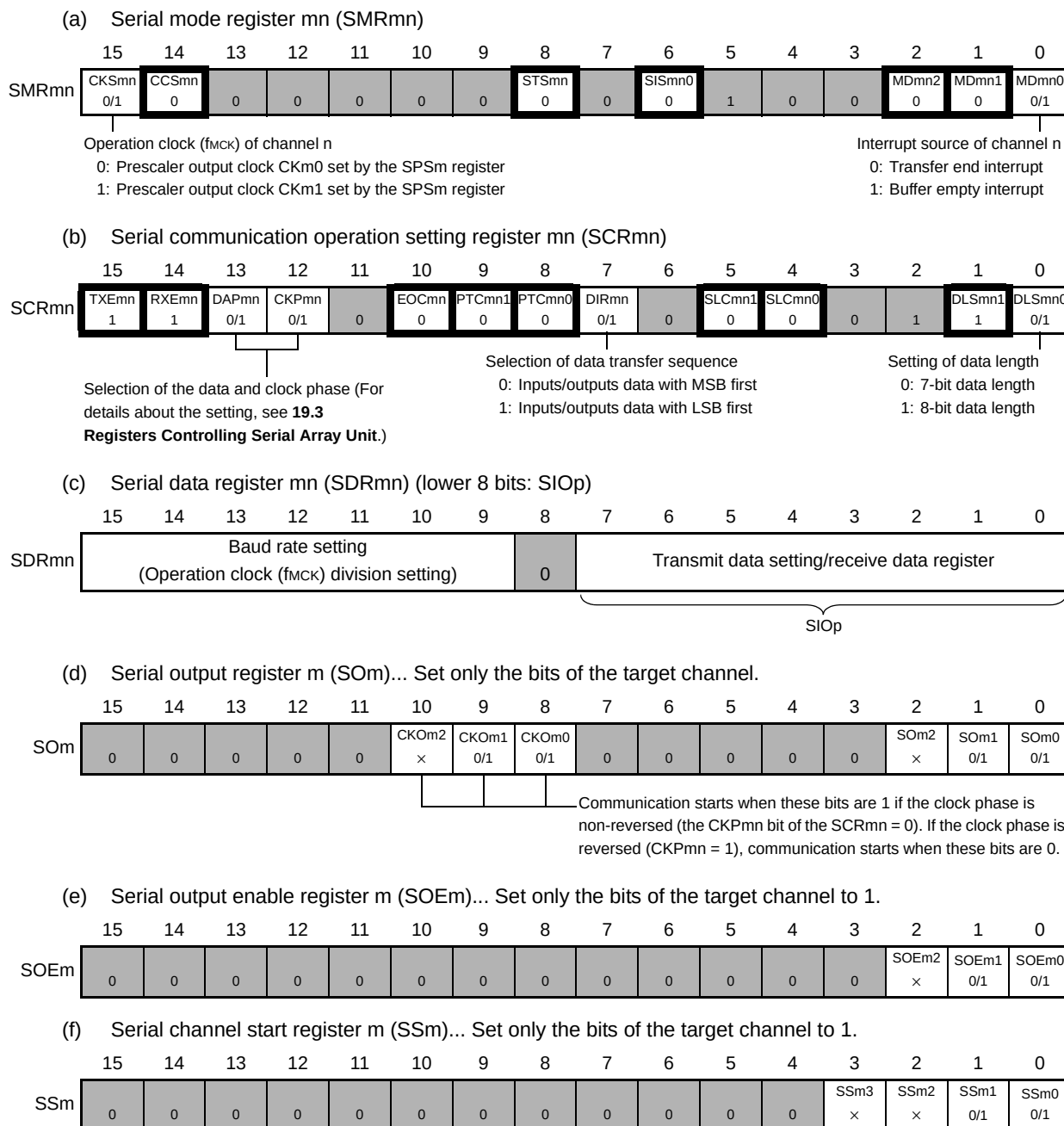
Figure 19 - 42 Example of Contents of Registers for Master Transmission/Reception of 3-Wire Serial I/O (CSI00, CSI01)
