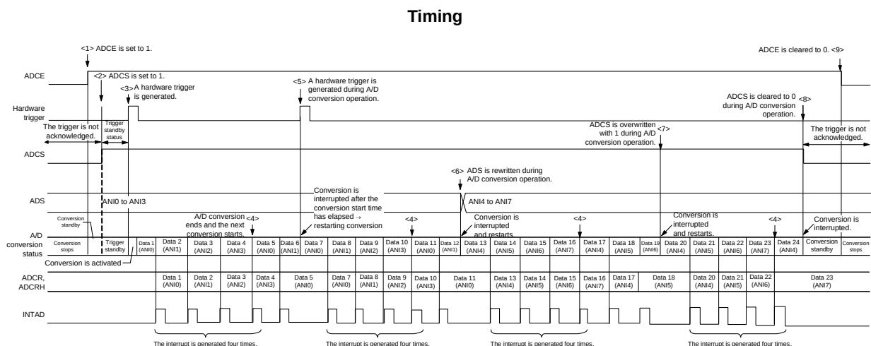
Figure 16 - 25 Example of Hardware Trigger No-Wait Mode (Scan Mode, Sequential Conversion Mode) Operation
