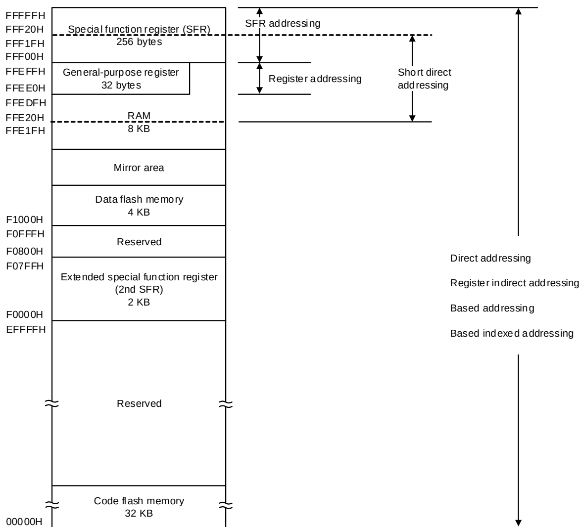
Figure 3 - 3 Correspondence Between Data Memory and Addressing
