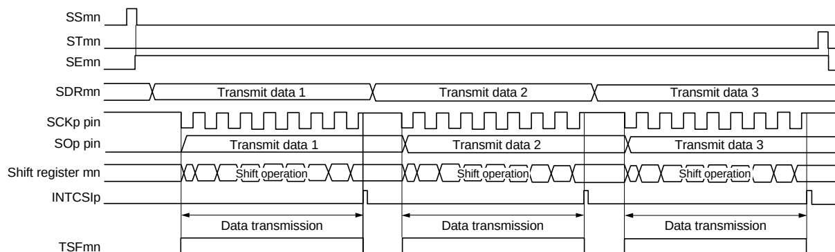
Figure 19 - 54 Timing Chart of Slave Transmission (in Single-Transmission Mode)
