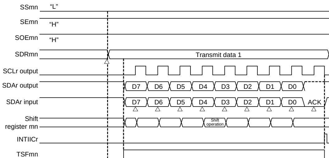
Figure 19 - 139 Timing Chart of Data Transmission
