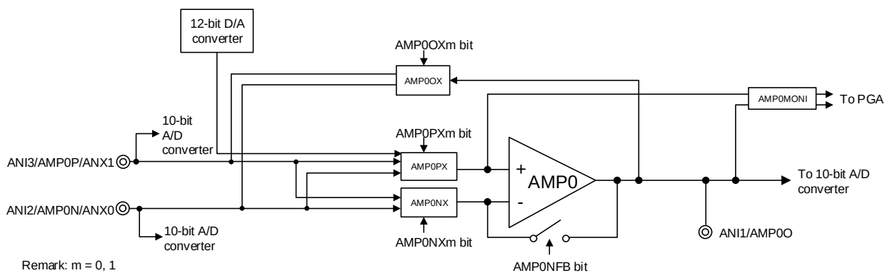
Figure 17 - 7 Block Diagram of Operational Amplifier 0
