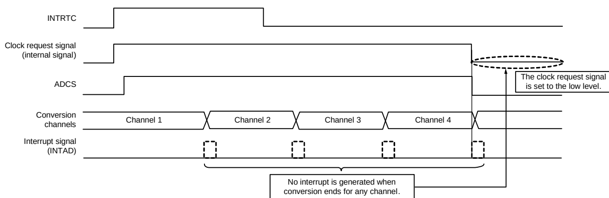
Figure 16 - 38 Operation Example When No Interrupt Is Generated After A/D Conversion Ends (While in Scan Mode)
