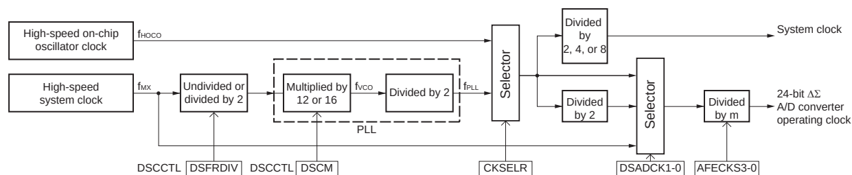
Figure 5 - 13 Relationship Between PLL and \Delta\Sigma A/D Converter
