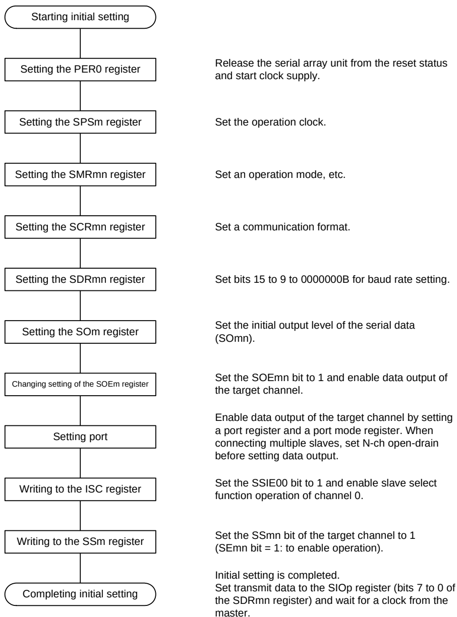
Figure 19 - 97 Initial Setting Procedure for Slave Transmission/Reception
