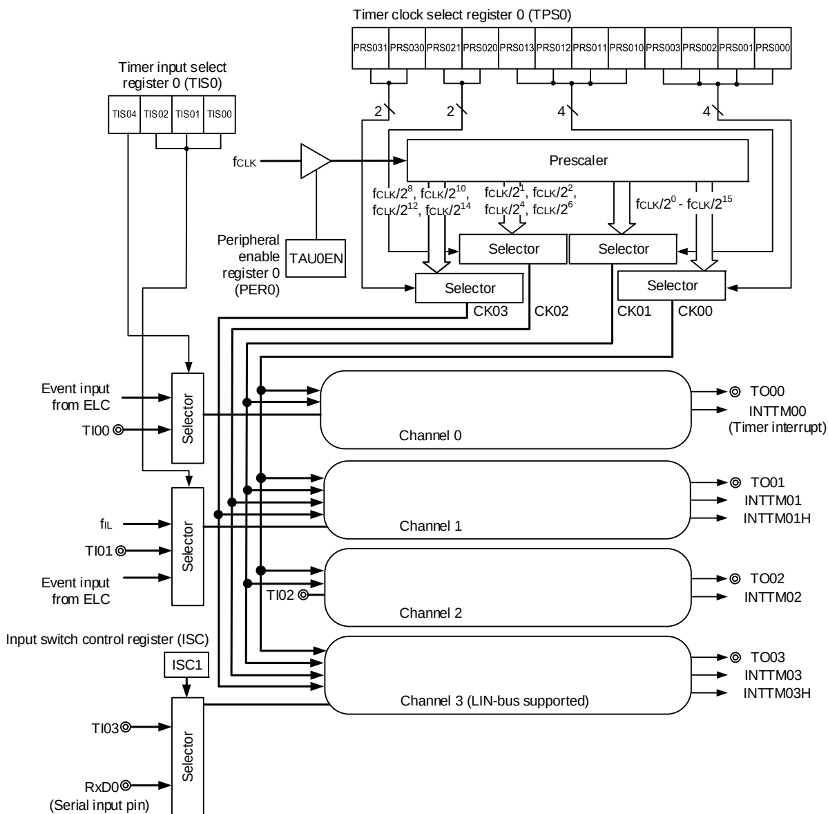
Figure 6 - 1 Entire Configuration of Timer Array Unit 0
