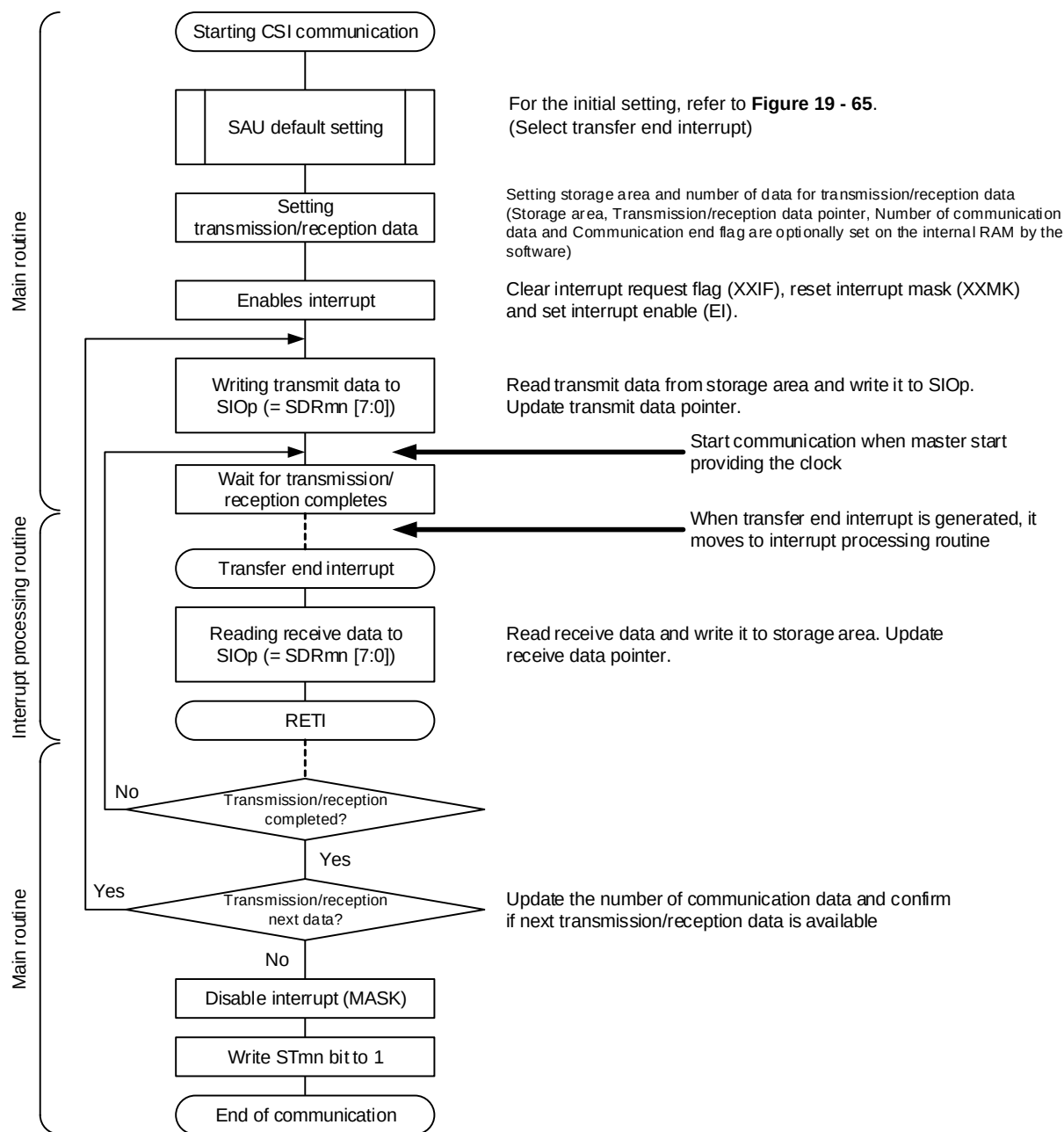
Figure 19 - 69 Flowchart of Slave Transmission/Reception (in Single- Transmission/Reception Mode)
