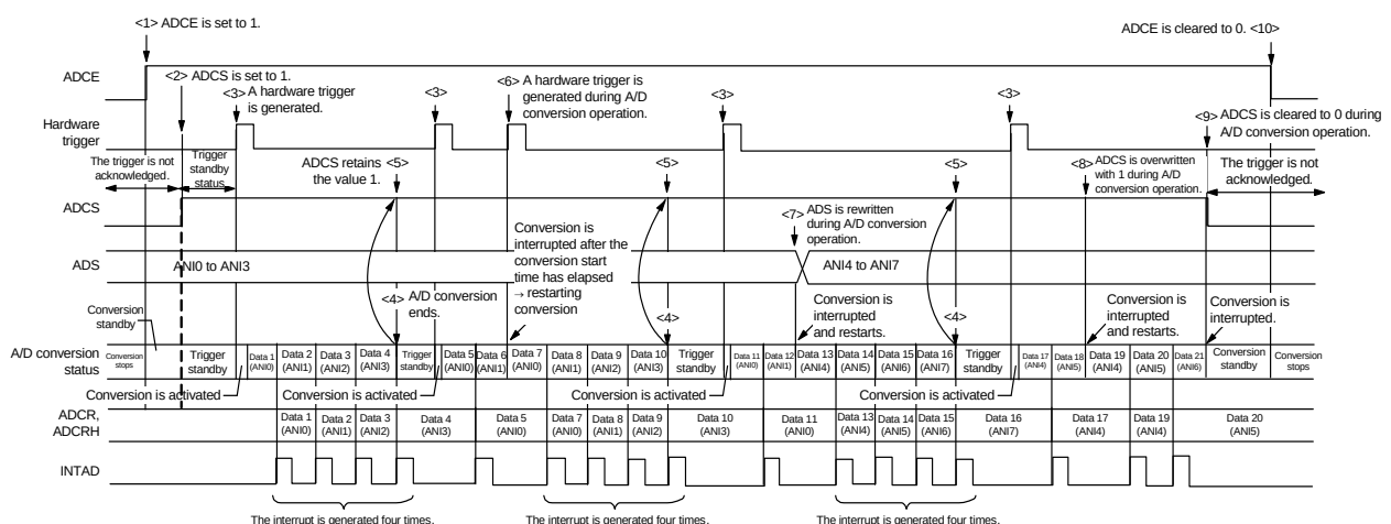
Figure 16 - 26 Example of Hardware Trigger No-Wait Mode (Scan Mode, One-Shot Conversion Mode) Operation Timing
