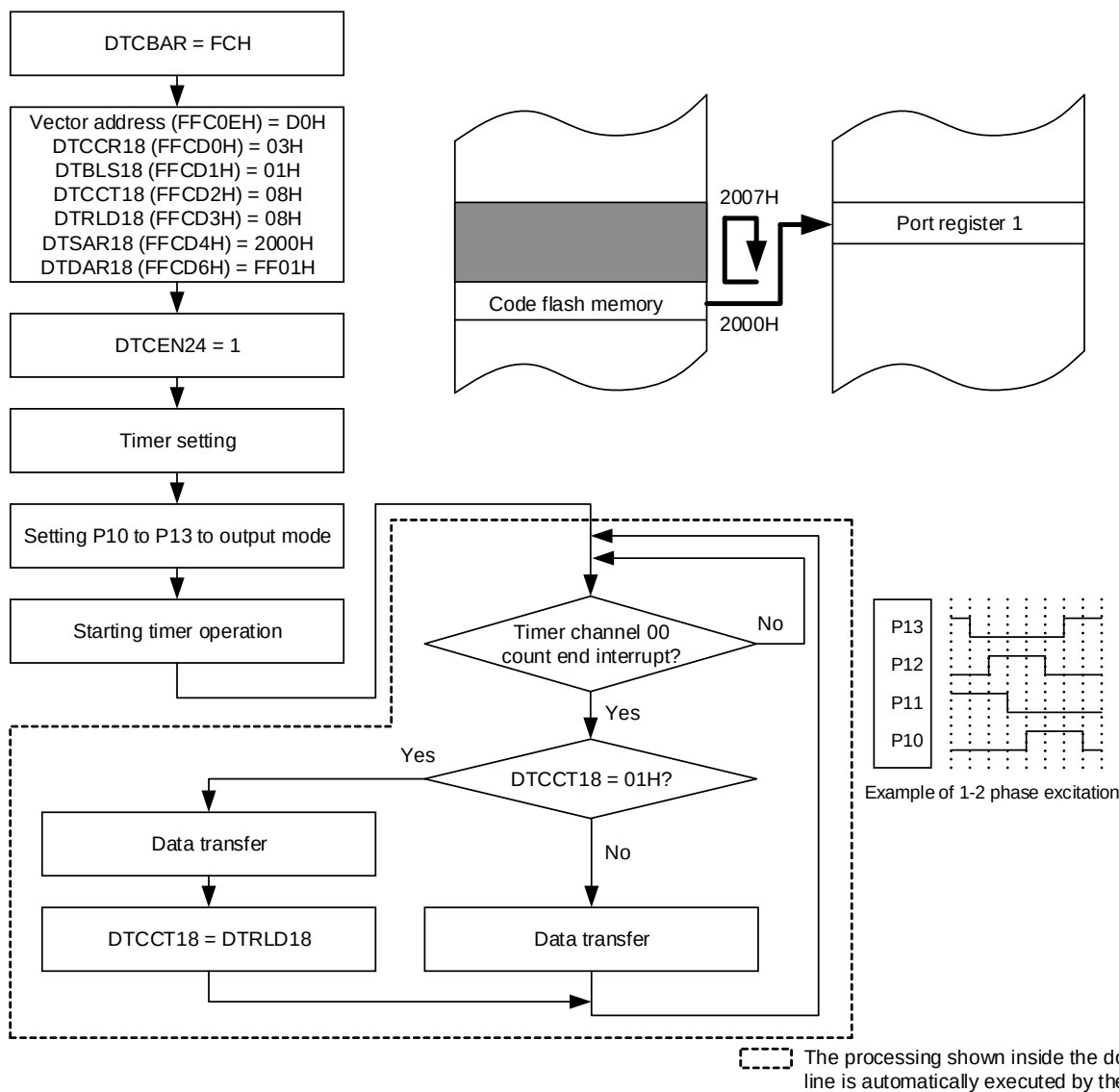
Figure 20 - 19 Example of using repeat mode - 1: Outputting a stepping motor control pulse using ports
