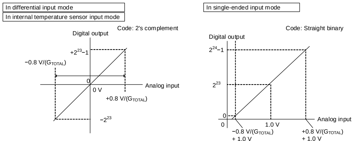
Figure 14 - 13 Voltage Input to the 24-bit \Delta\Sigma A/D Converter and A/D Conversion Result
