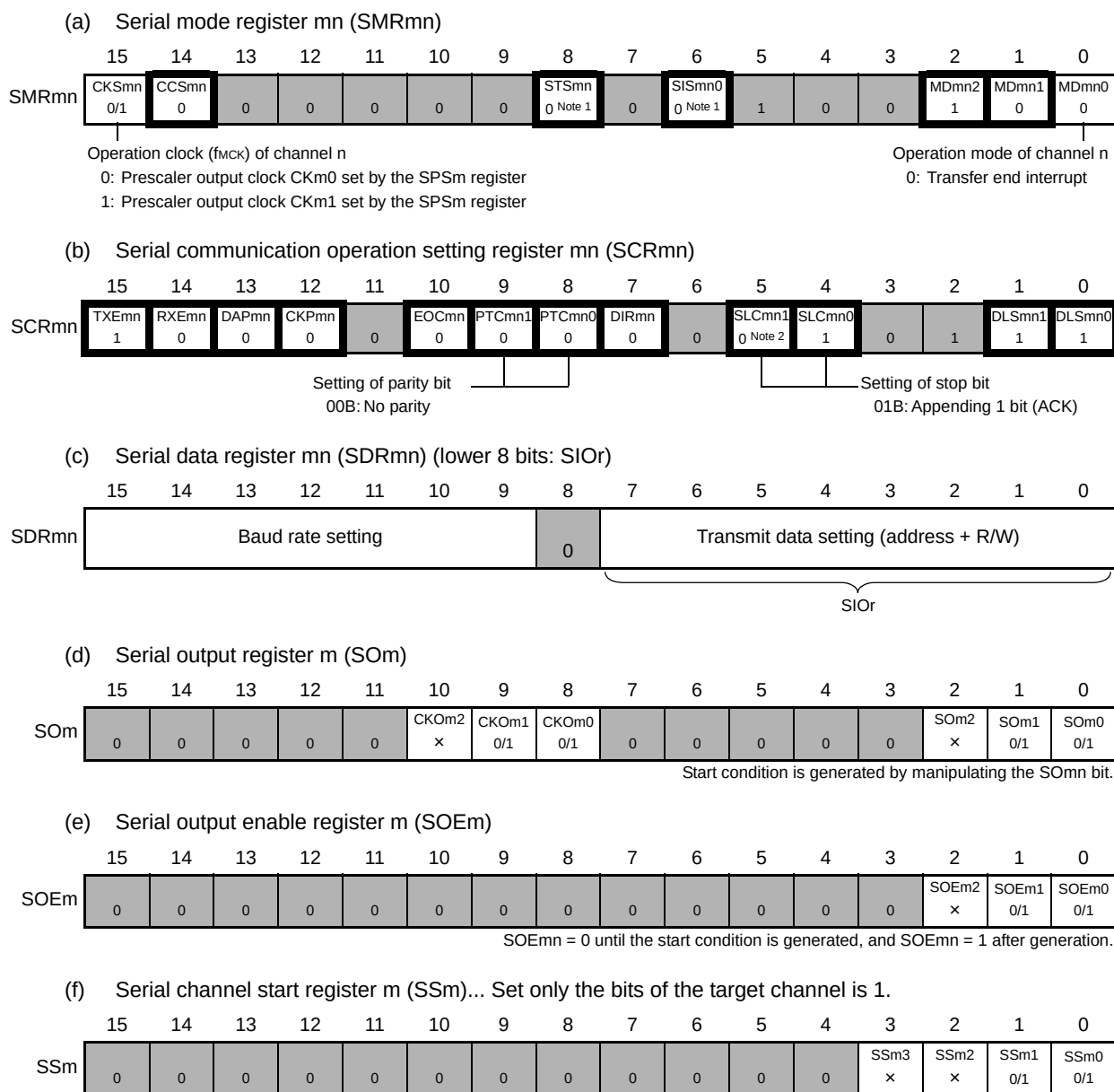
Figure 19 - 134 Example of Contents of Registers for Address Field Transmission of Simplified I 2 C (IIC00, IIC01)
