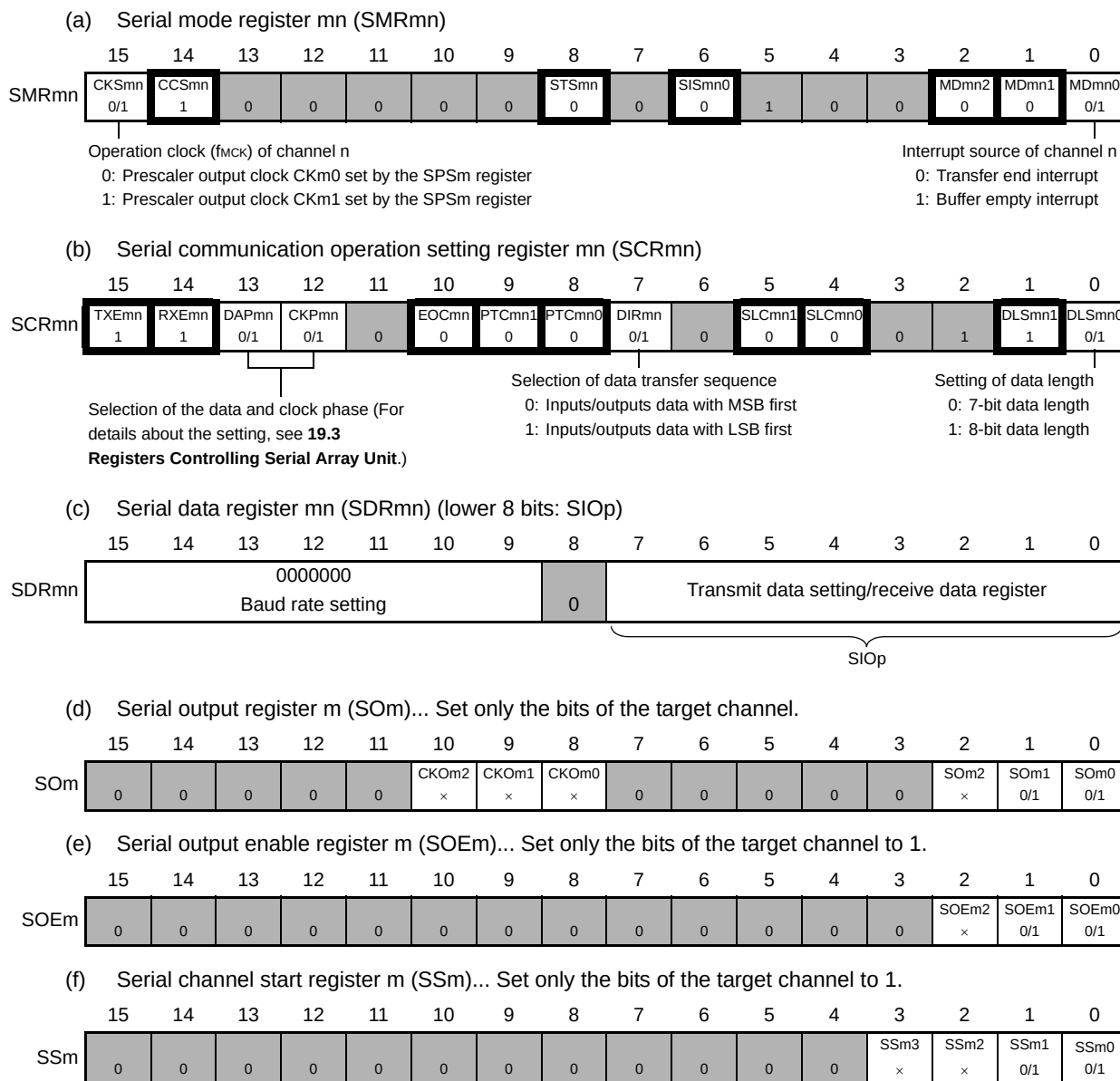
Figure 19 - 64 Example of Contents of Registers for Slave Transmission/Reception of 3-Wire Serial I/O (CSI00, CSI01)
