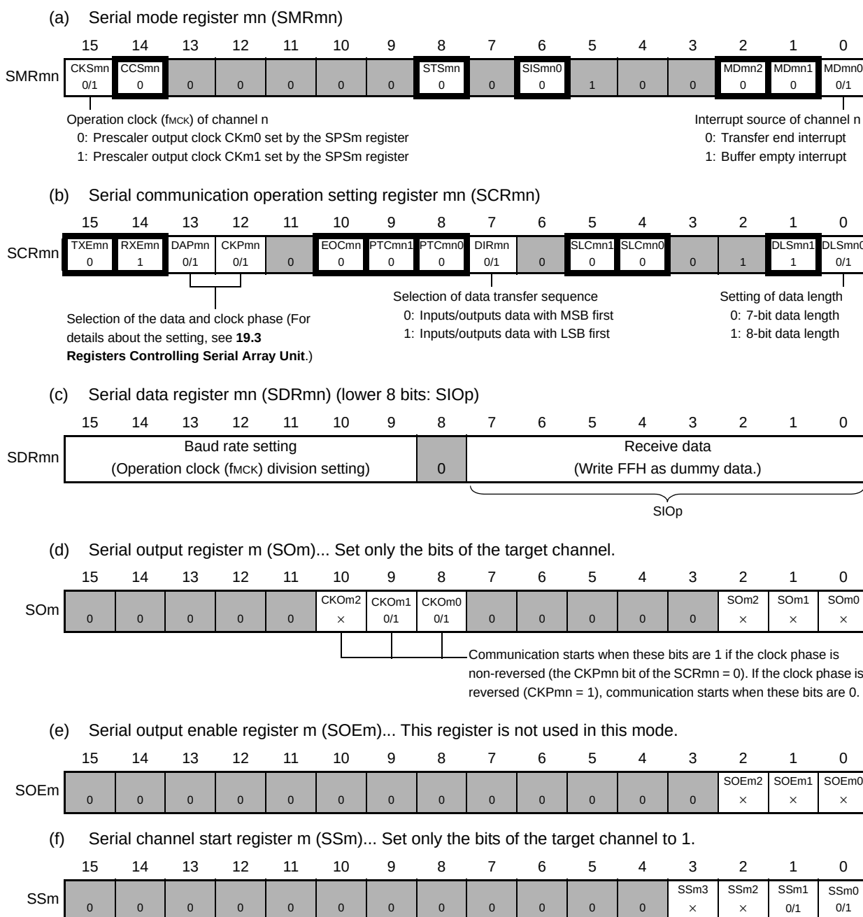
Figure 19 - 34 Example of Contents of Registers for Master Reception of 3-Wire Serial I/O (CSI00, CSI01)
