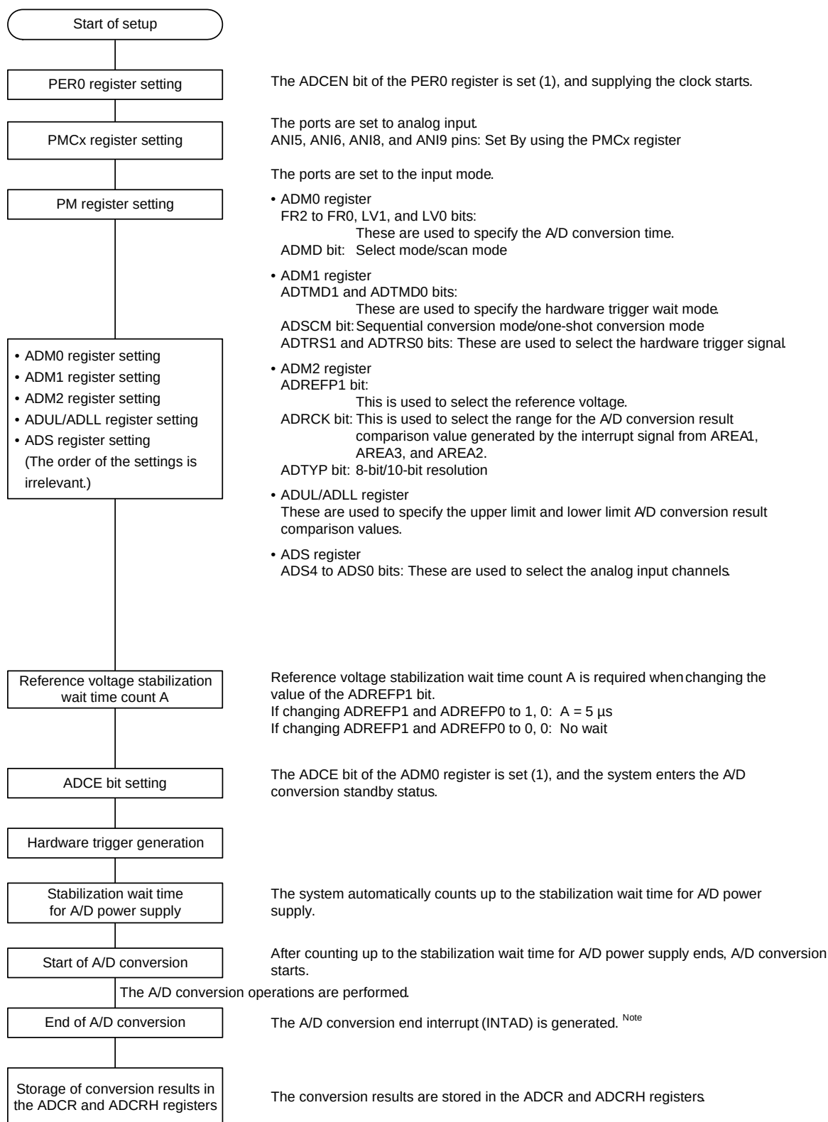
Figure 16 - 33 Setting up Hardware Trigger Wait Mode
