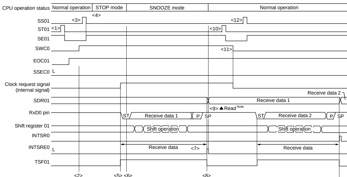
Figure 19 - 122 Timing Chart of SNOOZE Mode Operation (EOCm1 = 1, SSECm = 0)
