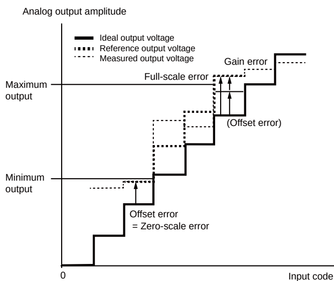
Figure 18 - 8 Relationship Between the Digital Inputs and Analog Outputs
