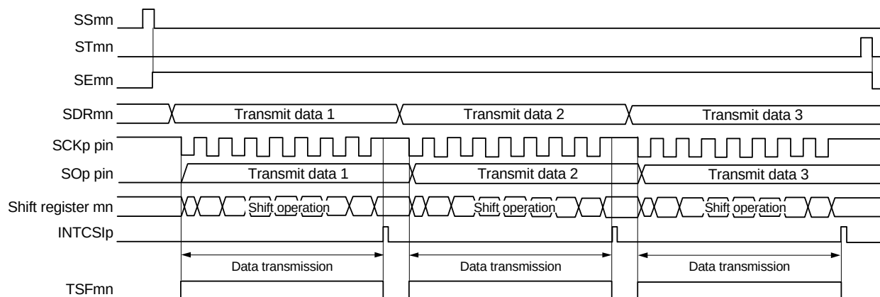
Figure 19 - 30 Timing Chart of Master Transmission (in Single-Transmission Mode)
