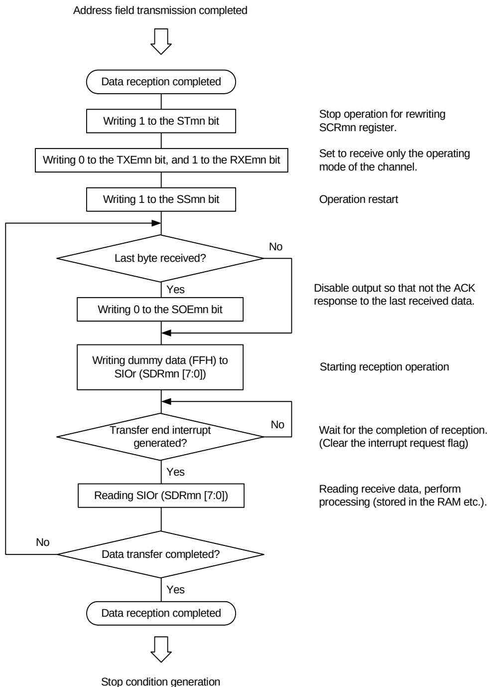
Figure 19 - 143 Flowchart of Data Reception
