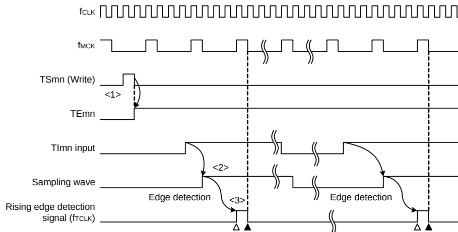
Figure 6 - 31 Timing of f CLK and count clock (f CLK ) (When CCSmn = 1, noise filter unused)
