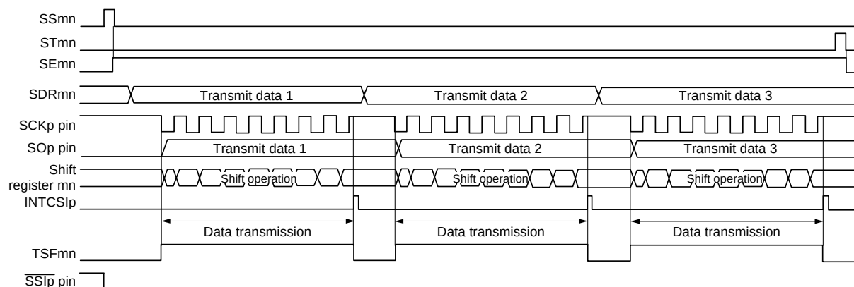
Figure 19 - 84 Timing Chart of Slave Transmission (in Single-Transmission Mode)
