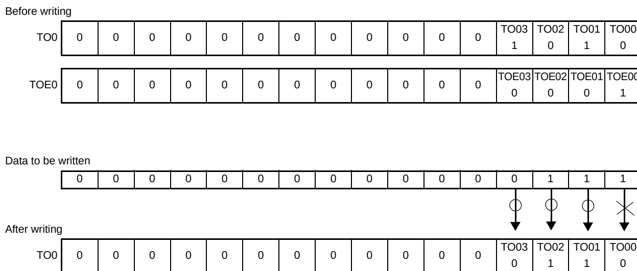
Figure 6 - 43 Example of TO0n Bit Collective Manipulation
