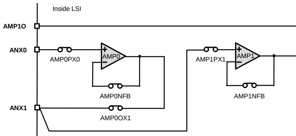
Figure 17 - 2 Example of Using a Configurable Amplifier as a Cascaded Voltage Follower
