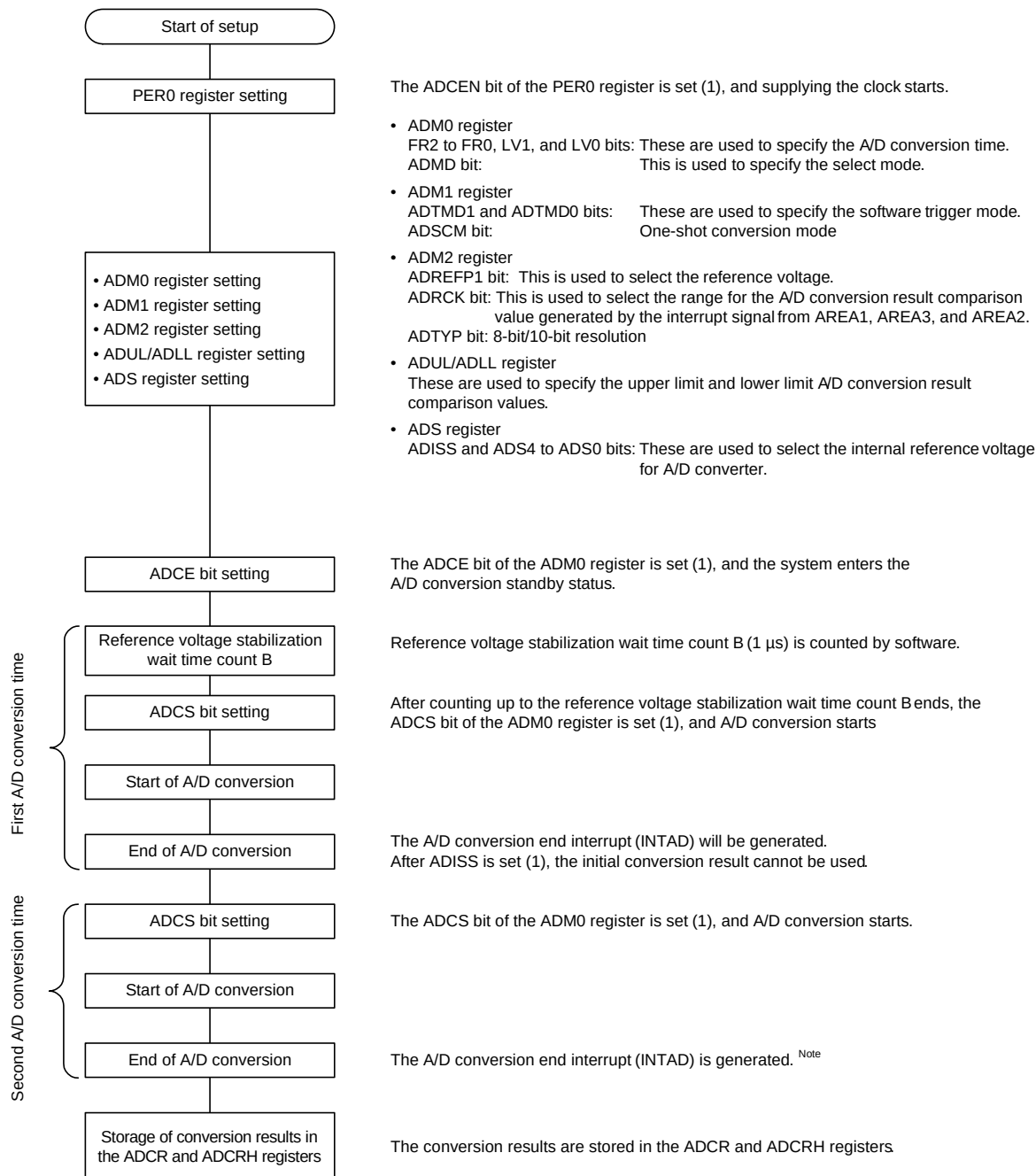
Figure 16 - 34 Setup when internal reference voltage for A/D converter is selected
