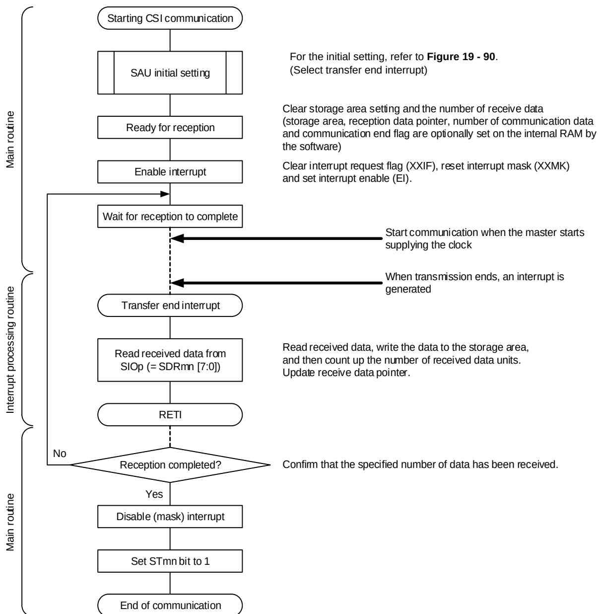
Figure 19 - 94 Flowchart of Slave Reception (in Single-Reception Mode)
