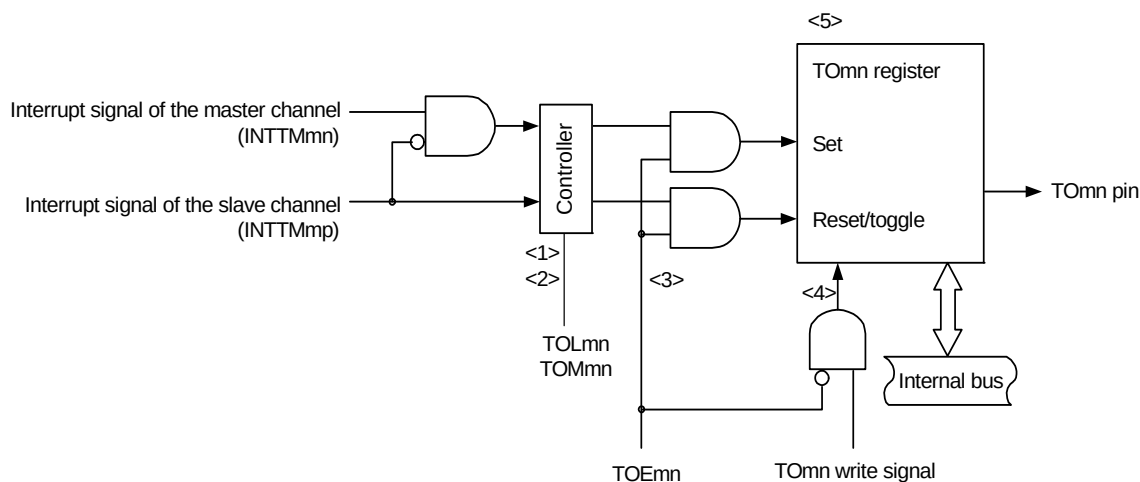
Figure 6 - 37 Output Circuit Configuration
