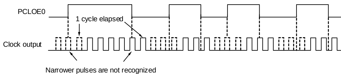
Figure 11 - 3 Timing of Outputting Clock from PCLBUZ0 Pin
