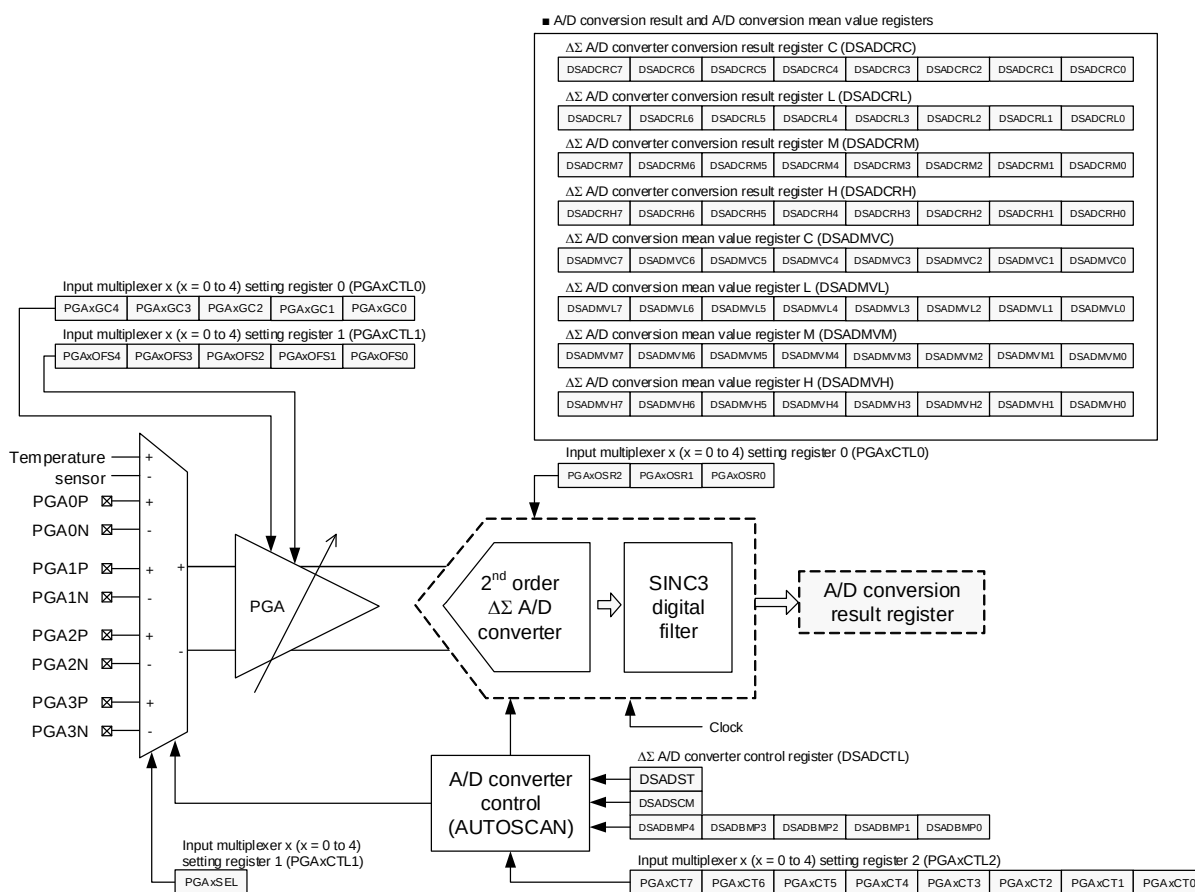
Figure 14 - 12 Block Diagram of 24-bit \Delta\Sigma A/D Converter
