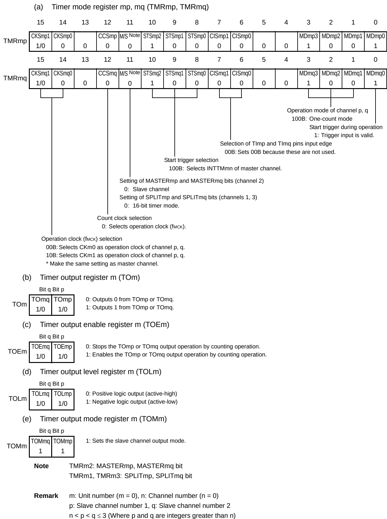
Figure 6 - 84 Example of Set Contents of Registers When Multiple PWM Output Function (Slave Channel) Is Used (output two types of PWMs)
