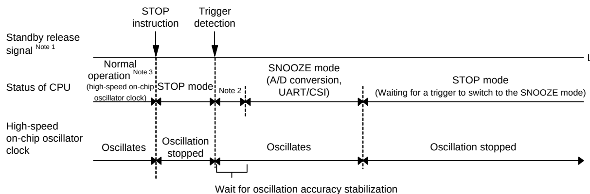
Figure 23 - 7 When the Interrupt Request Signal is not Generated in the SNOOZE Mode
