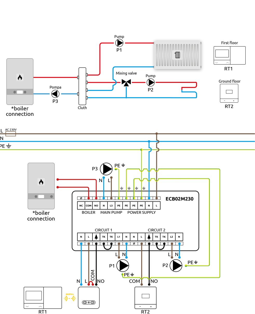
a) - Connection of 2 heating circuits
