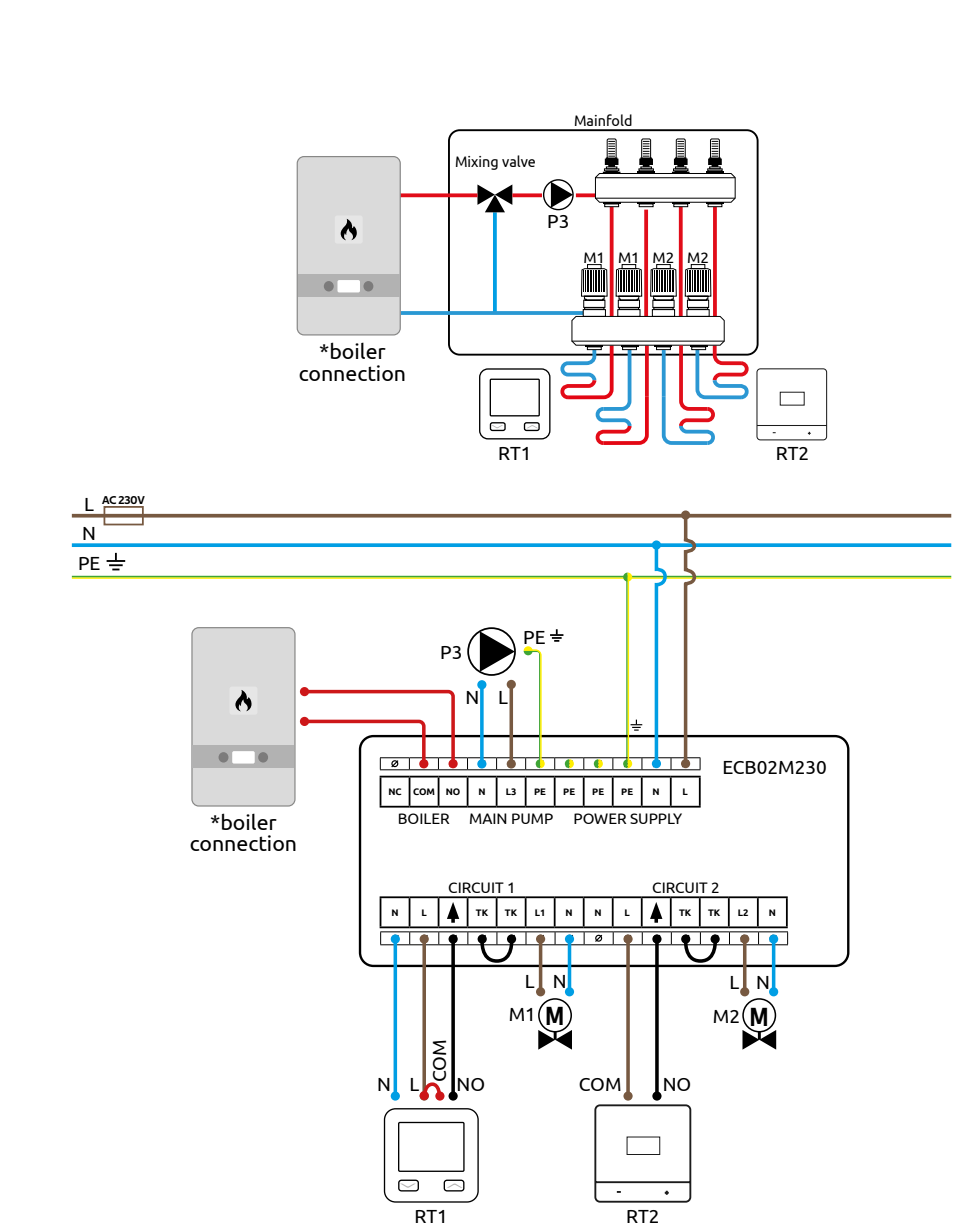
b) - Connection of 2 underfloor heating zones
