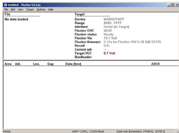
Figure 56. Incorrect Target VCC Value
