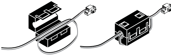
Figure 5. Clamp-On Ferrite Bead Installation
