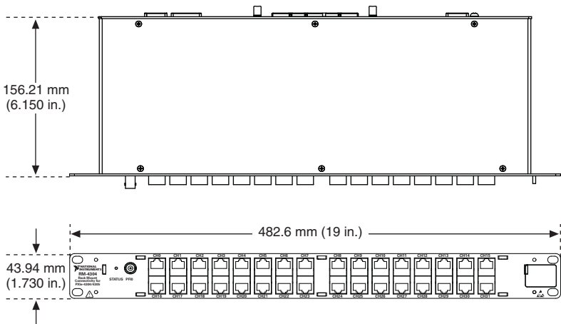
Figure 10. RM-4304 Dimensions
